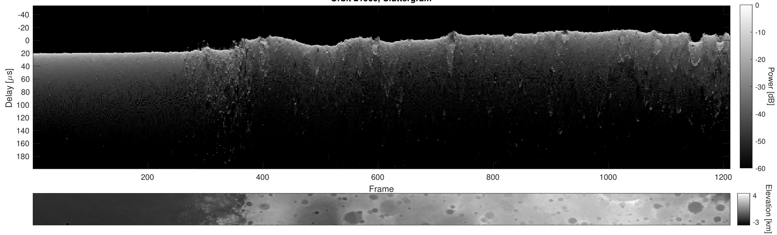
Orbit 21960, Cluttergram
