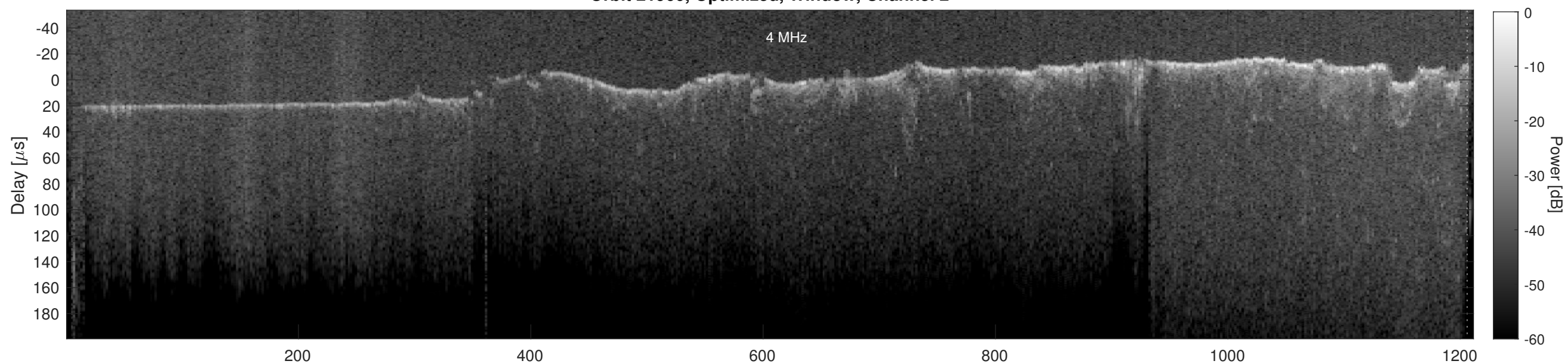
Orbit 21960, Cluttergram
