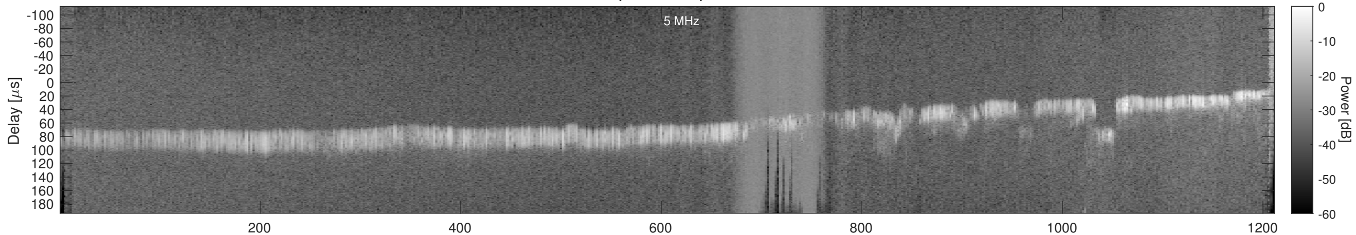
Orbit 21961, Window, Channel 1, Chapman
