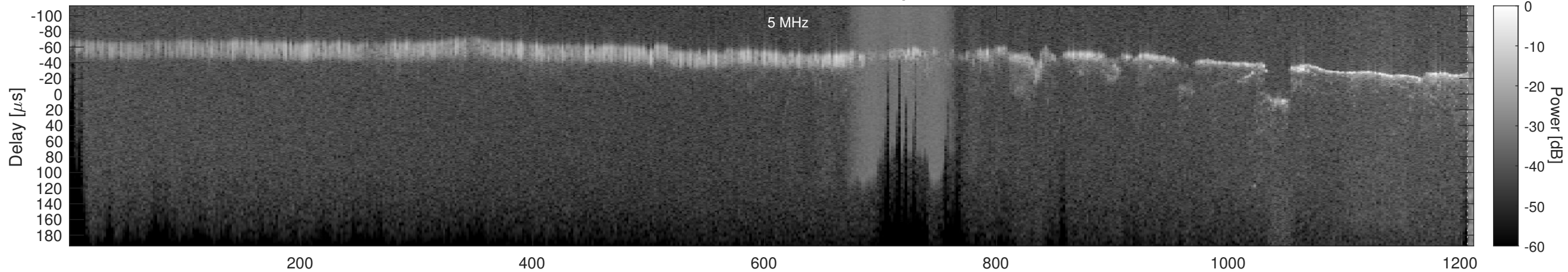
Orbit 21961, Window, Channel 1, Optimized
