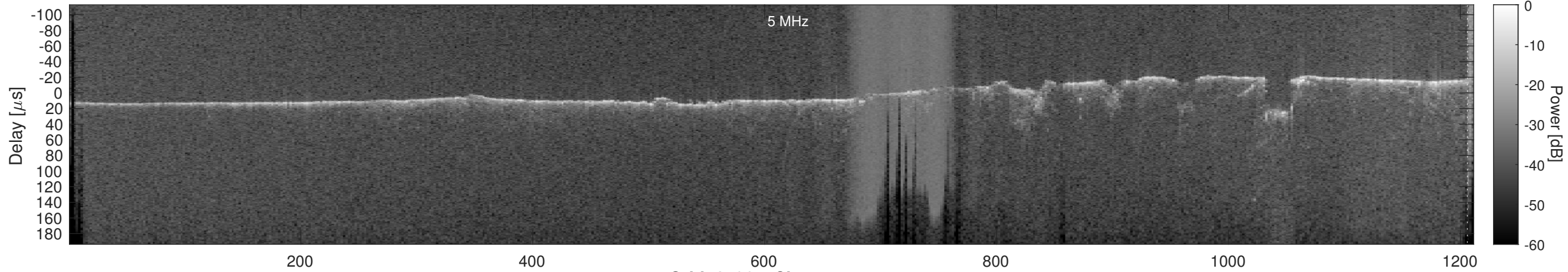
Orbit 21961, Cluttergram
