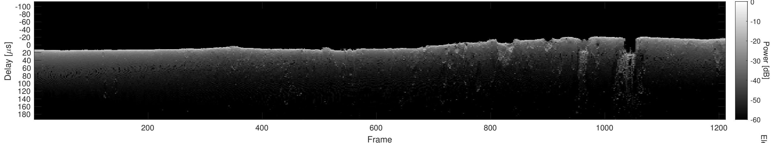
Orbit 21961, Cluttergram
