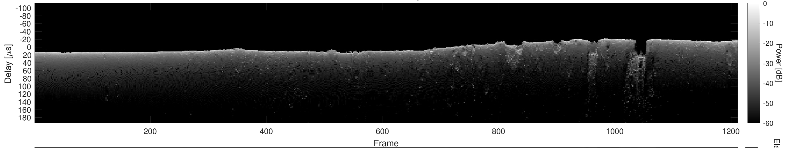
Orbit 21961, Cluttergram
