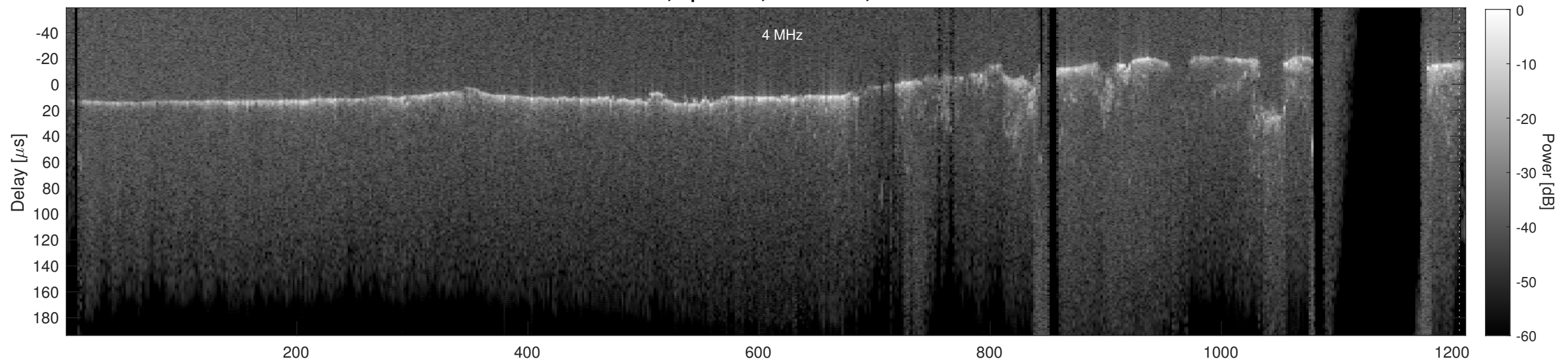
Orbit 21961, Cluttergram
