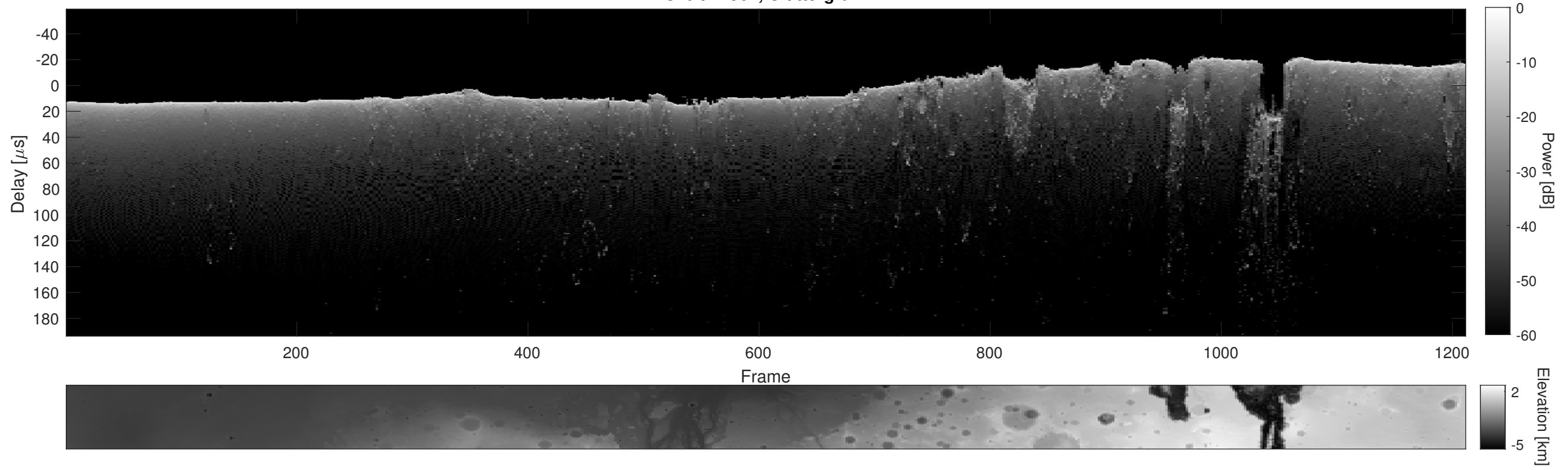
Orbit 21961, Cluttergram
