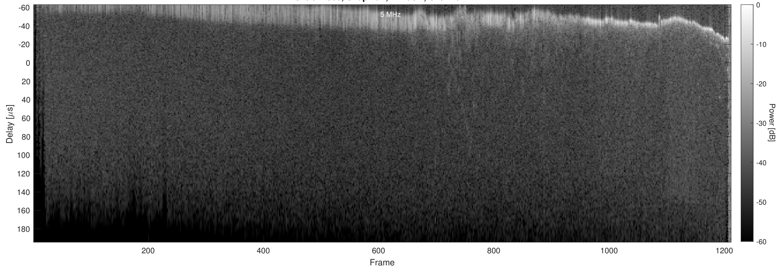
Orbit 21963, Chapman, Window, Channel 2
