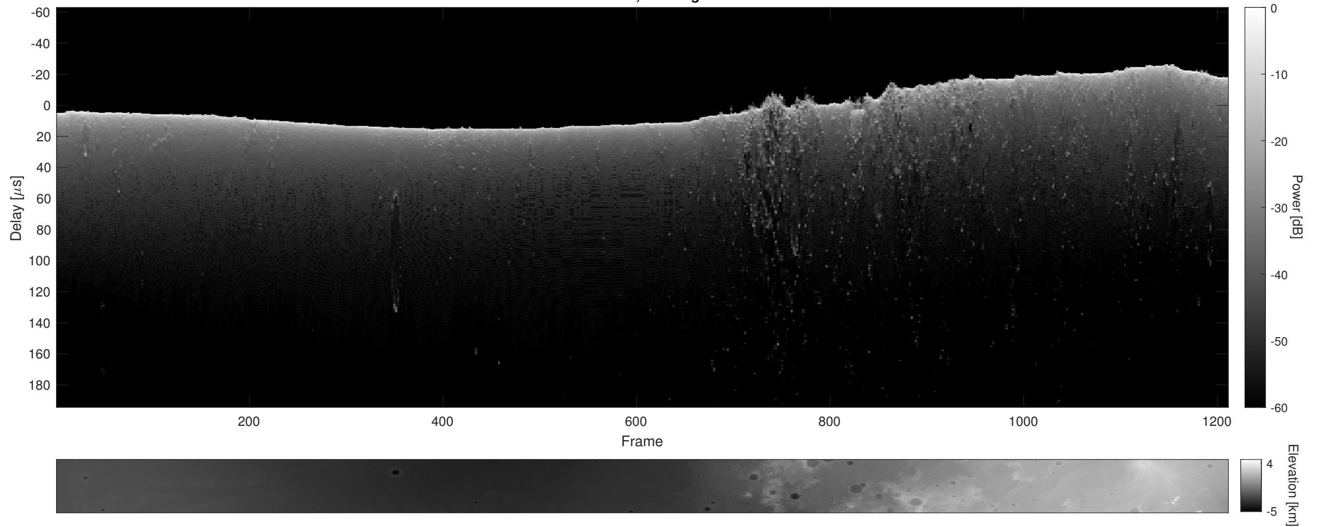
Orbit 21963, Cluttergram
