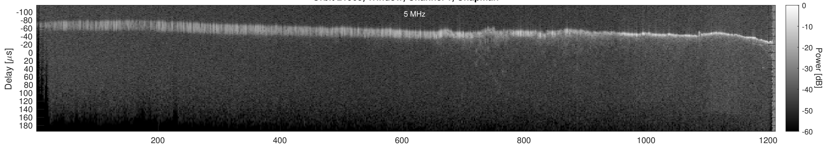
Orbit 21963, Window, Channel 1, Optimized
