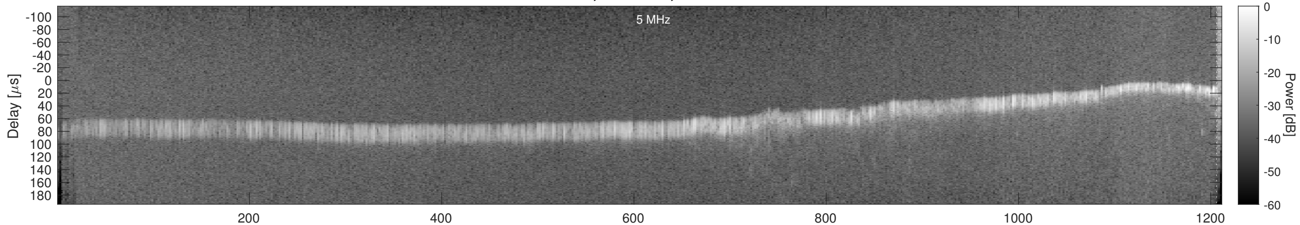
Orbit 21963, Window, Channel 1, Chapman
