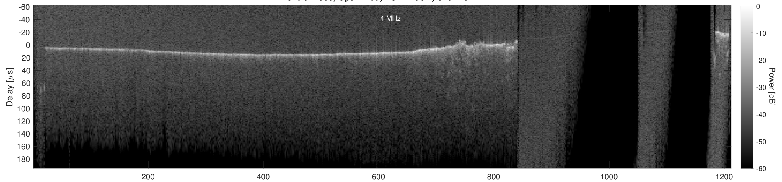
Orbit 21963, Cluttergram
