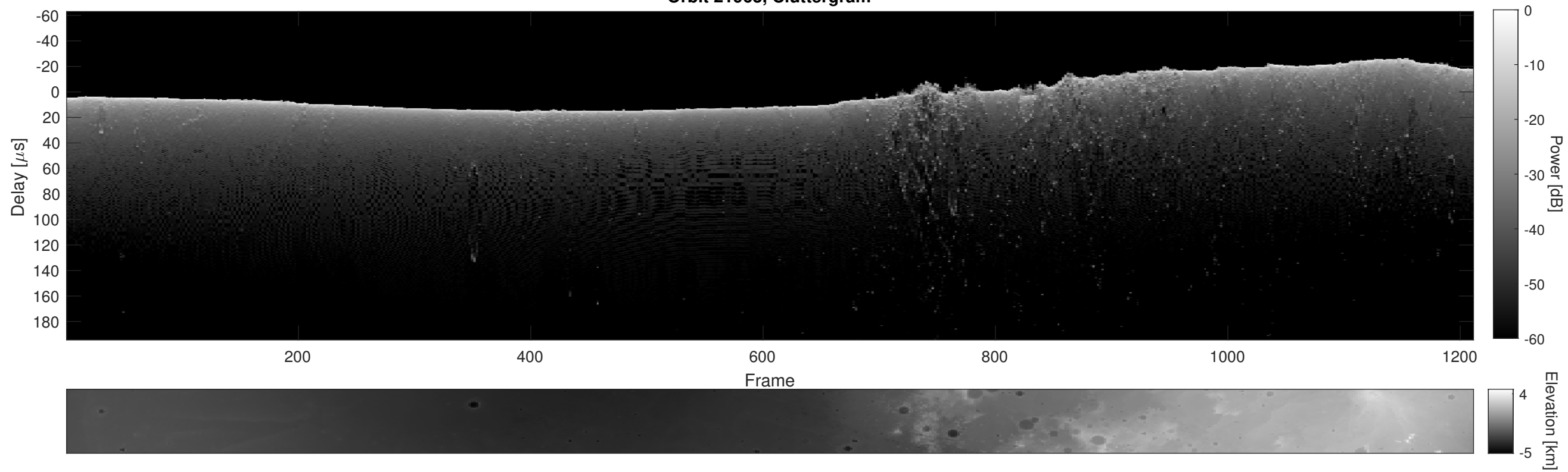
Orbit 21963, Cluttergram
