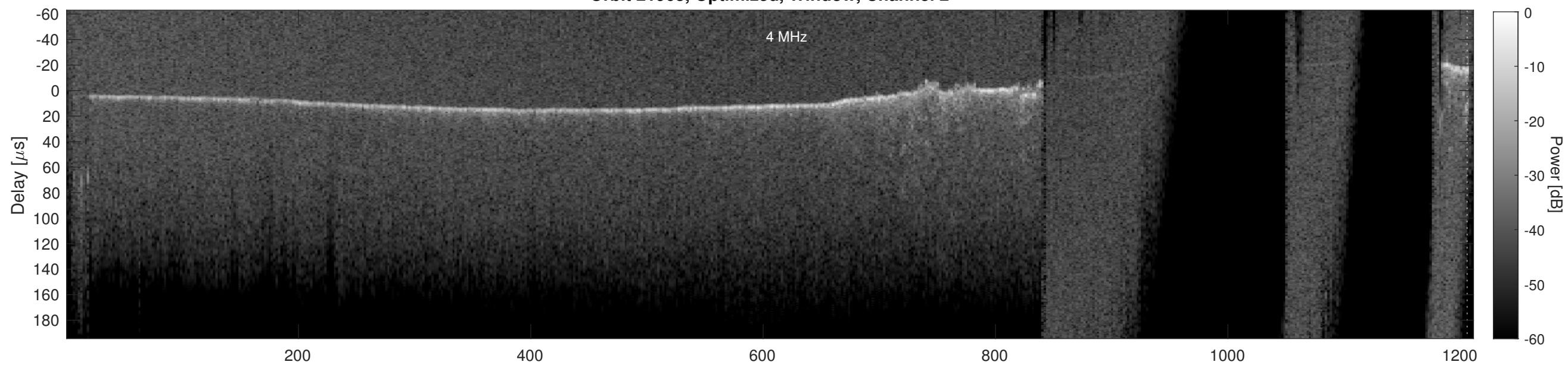
Orbit 21963, Cluttergram
