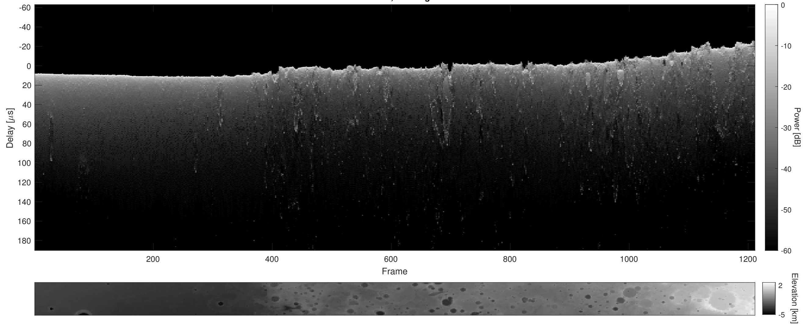
Orbit 21964, Cluttergram
