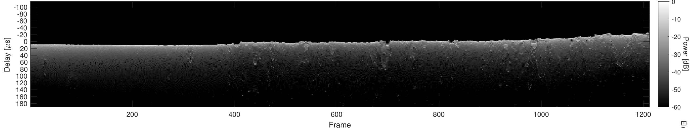
Orbit 21964, Cluttergram
