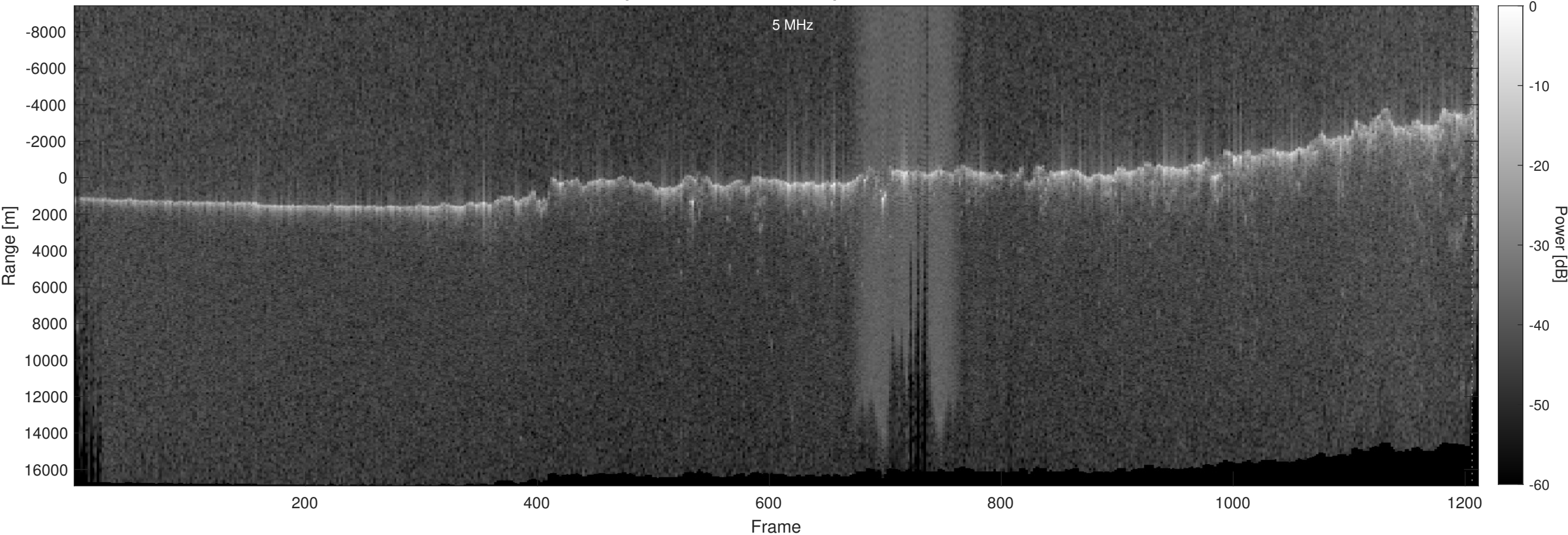
Orbit 21964, Optimized, No Window, Depth-Corrected, Channel 2
