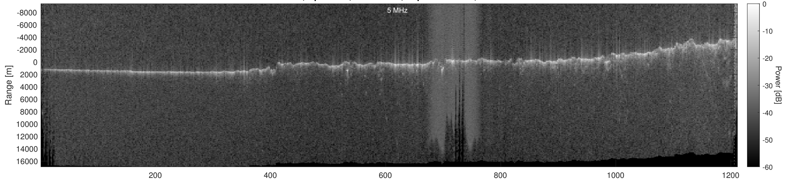
Orbit 21964, Optimized, No Window, Depth-Corrected, Channel 2
