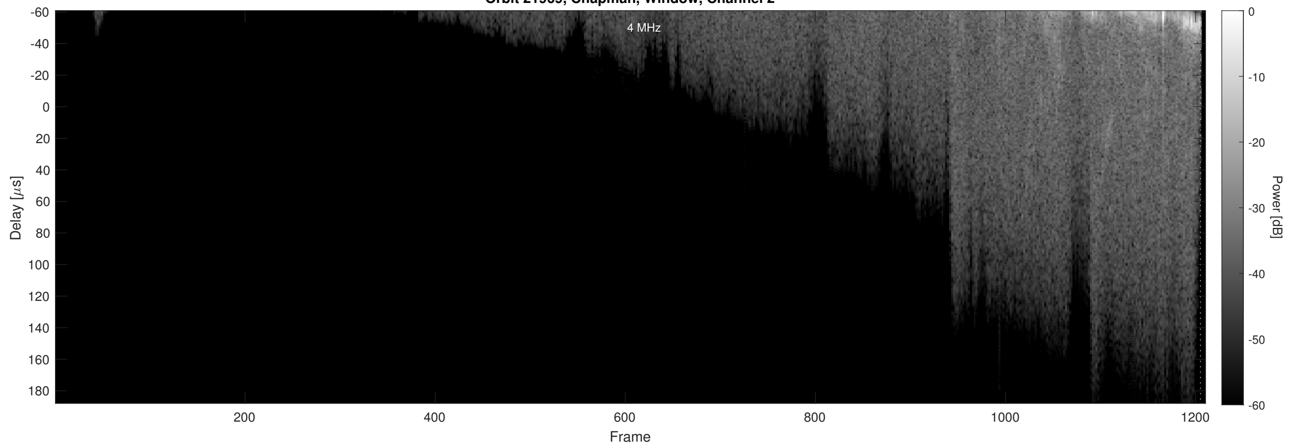
Orbit 21969, Chapman, Window, Channel 2
