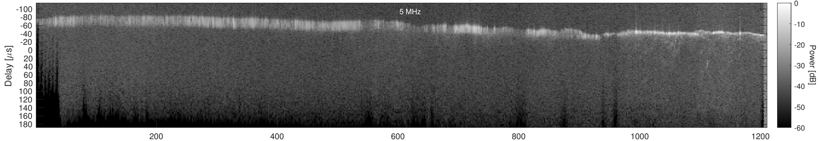
Orbit 21969, Window, Channel 1, Optimized
