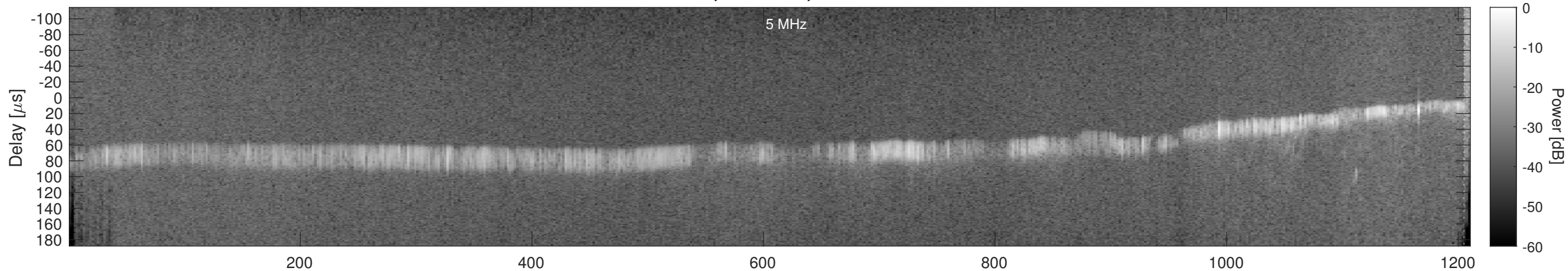
Orbit 21969, Window, Channel 1, Chapman
