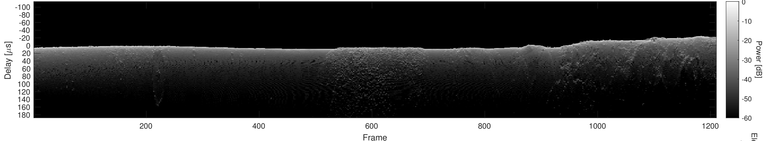
Orbit 21969, Cluttergram
