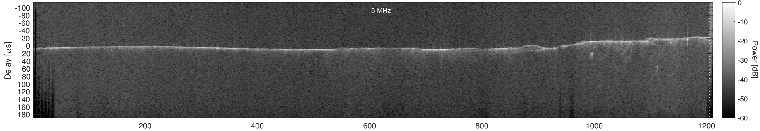
Orbit 21969, Cluttergram
