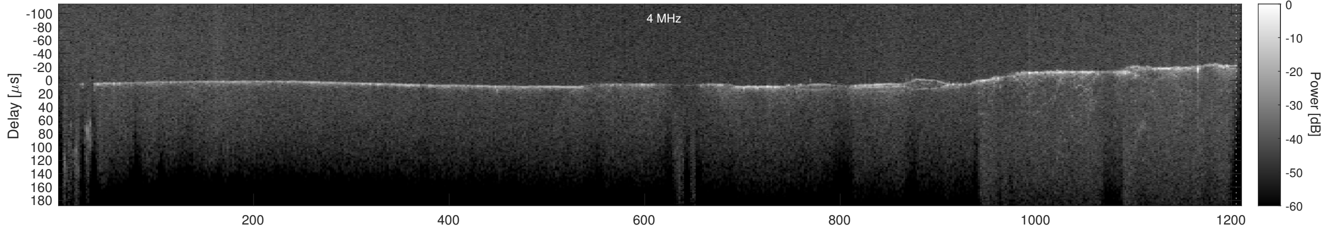
Orbit 21969, Cluttergram
