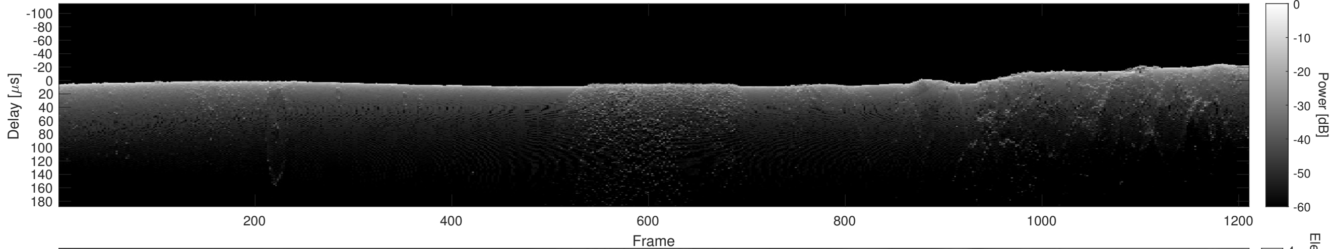
Orbit 21969, Cluttergram
