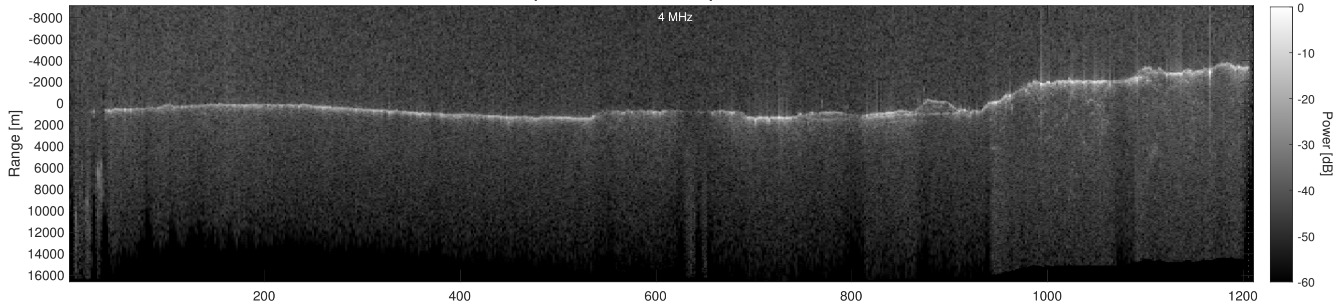
Orbit 21969, Depth-Corrected Cluttergram
