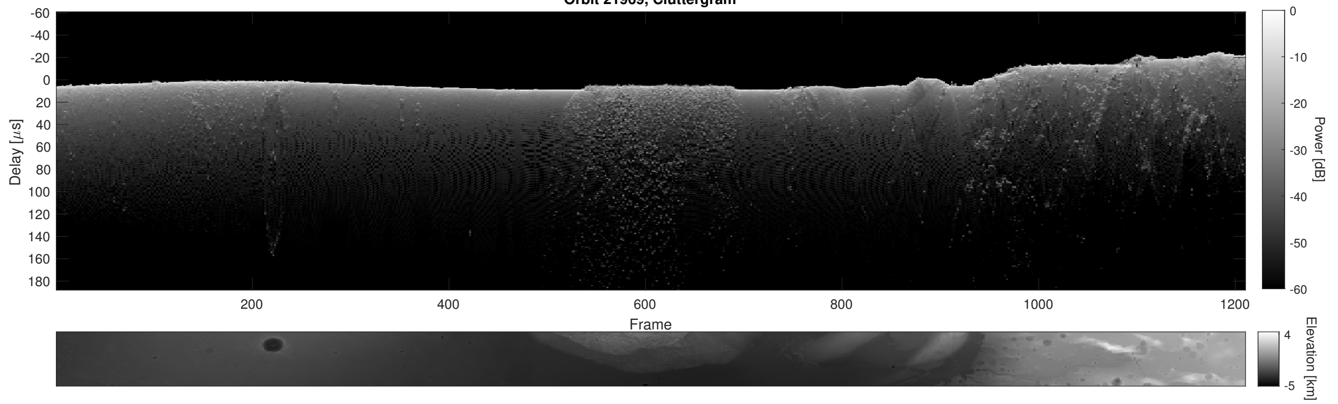
Orbit 21969, Cluttergram
