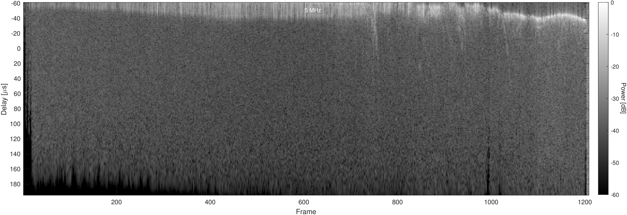
Orbit 21970, Chapman, No Window, Channel 2
