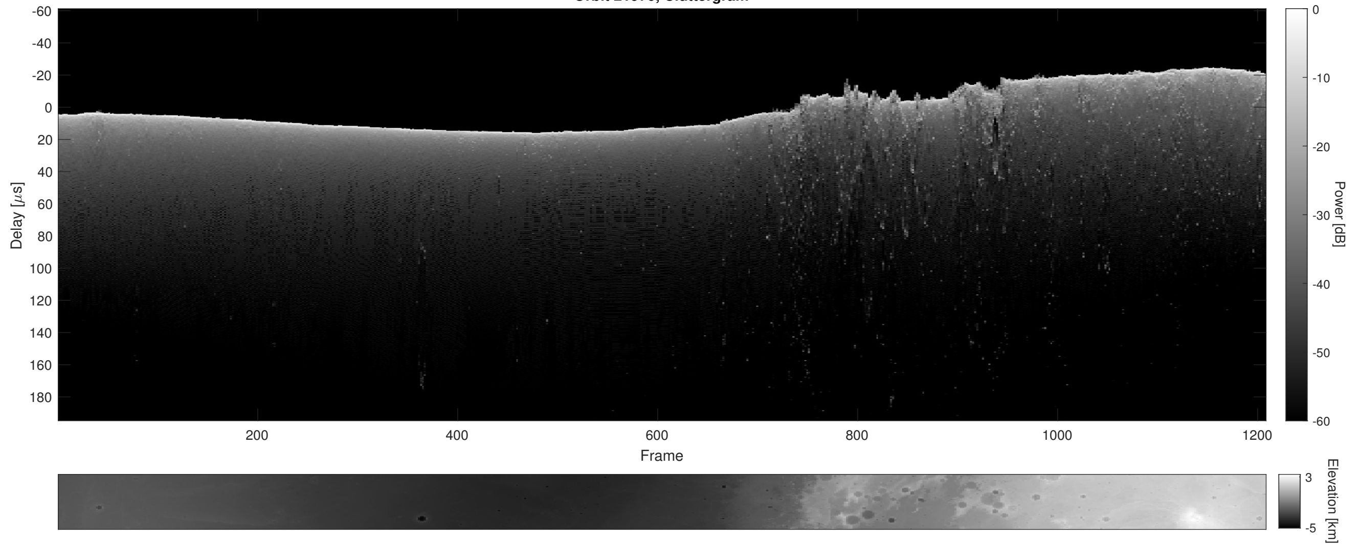
Orbit 21970, Cluttergram
