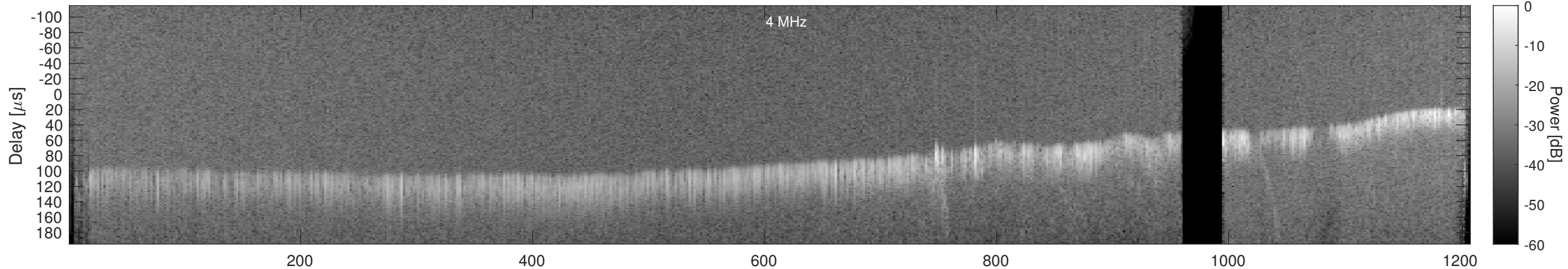
Orbit 21970, Window, Channel 2, Chapman
