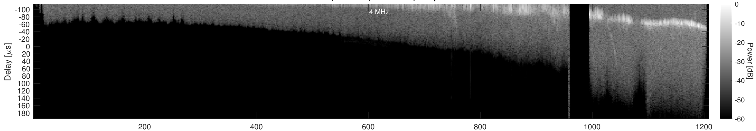
Orbit 21970, Window, Channel 2, Optimized
