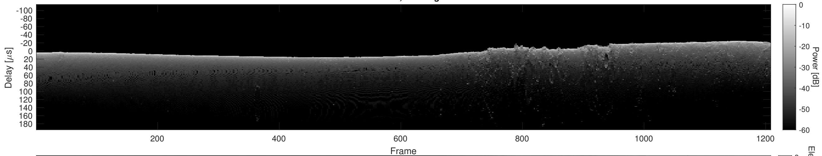
Orbit 21970, Cluttergram
