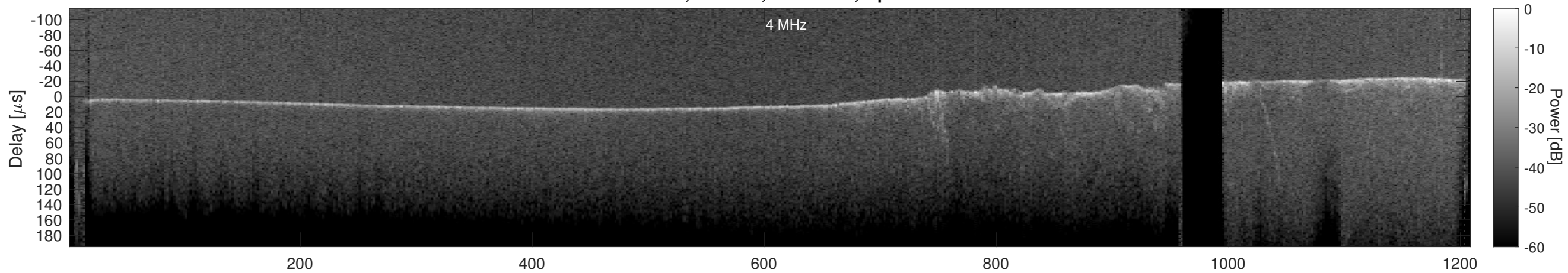
Orbit 21970, Cluttergram
