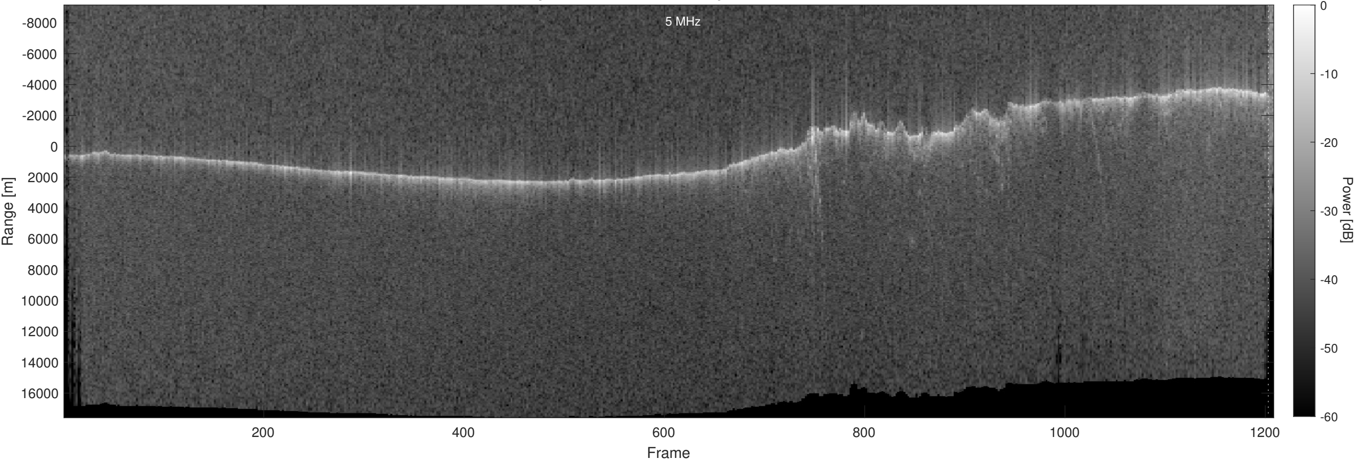
Orbit 21970, Optimized, No Window, Depth-Corrected, Channel 2
