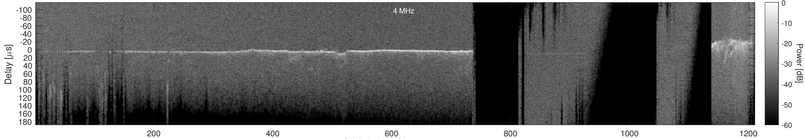
Orbit 21973, Cluttergram
