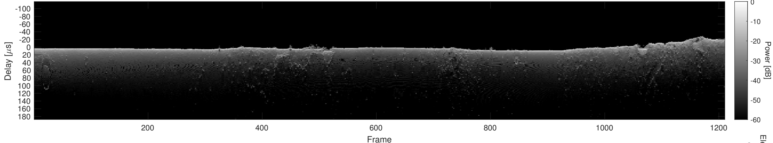
Orbit 21973, Cluttergram
