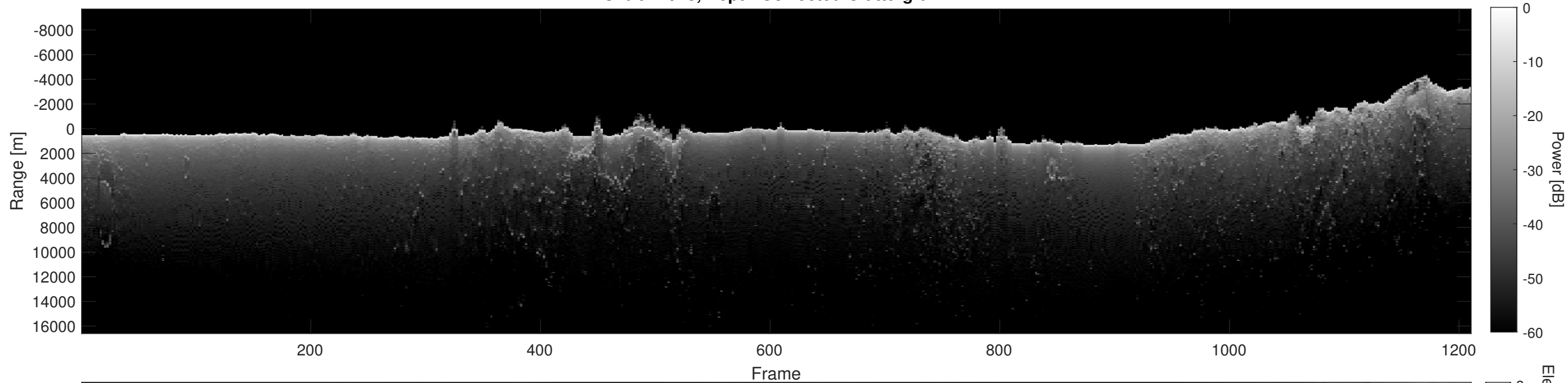
Orbit 21973, Depth-Corrected Cluttergram
