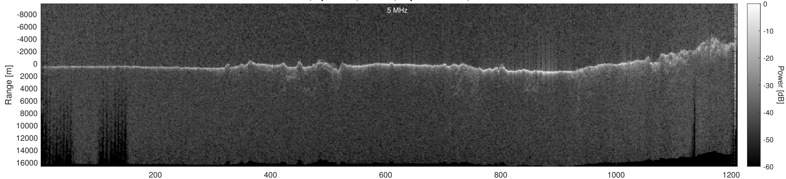
Orbit 21973, Optimized, Window, Depth-Corrected, Channel 2
