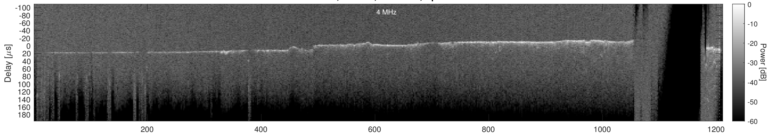
Orbit 21974, Cluttergram
