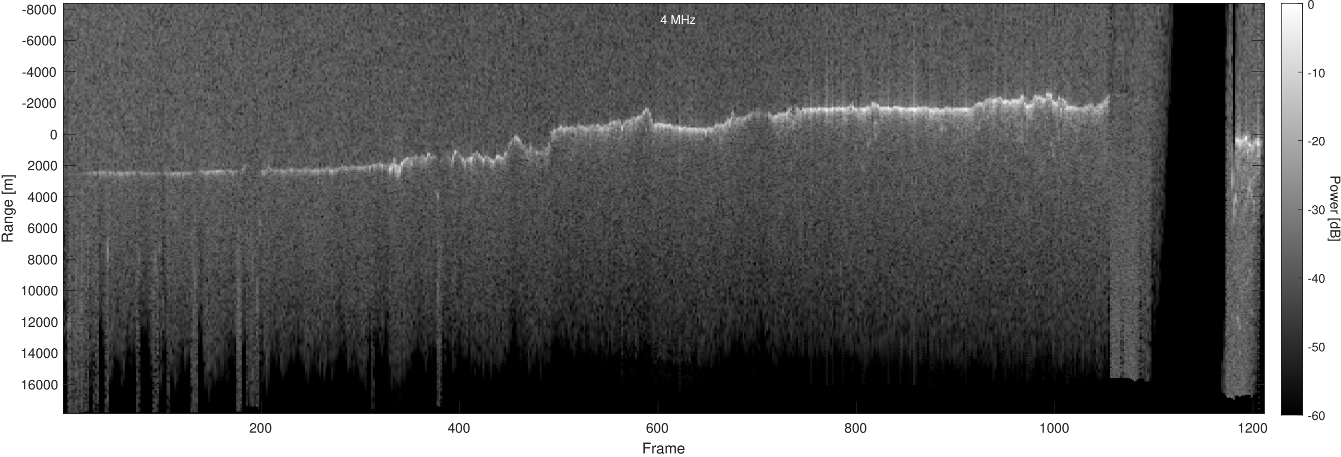
Orbit 21974, Optimized, No Window, Depth-Corrected, Channel 2
