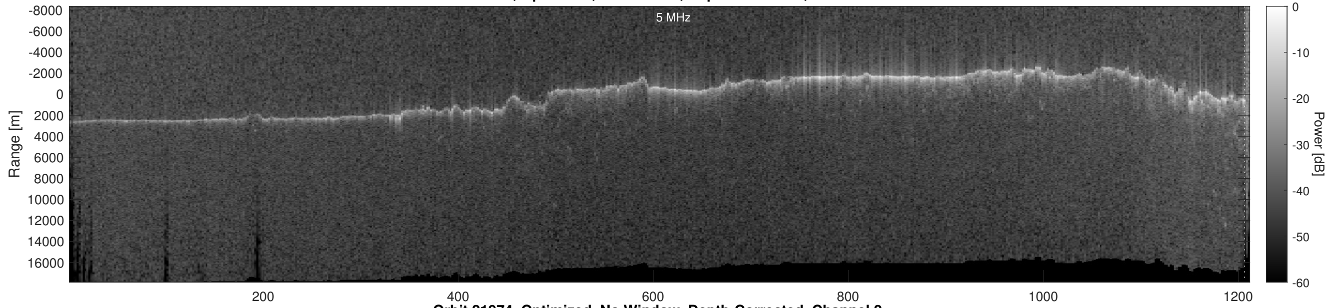
Orbit 21974, Optimized, No Window, Depth-Corrected, Channel 2
