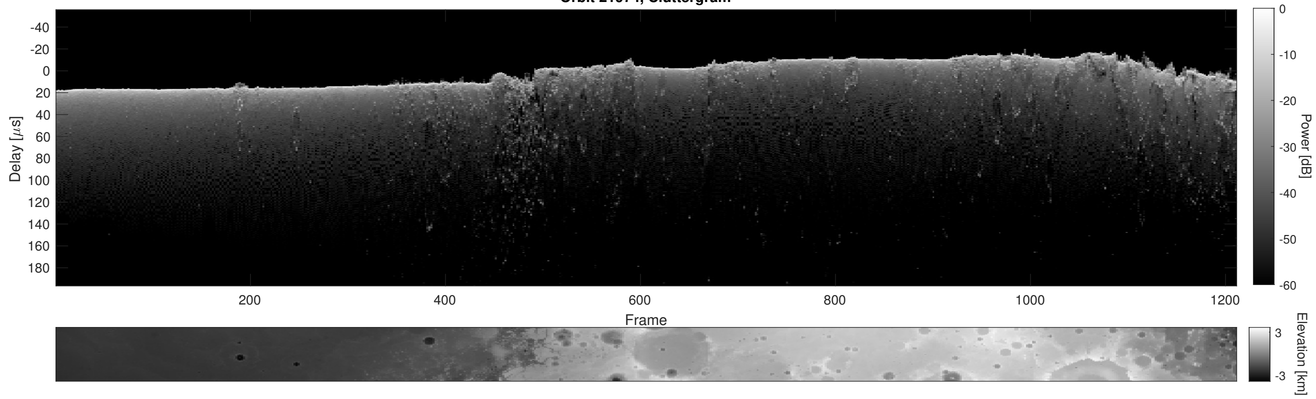
Orbit 21974, Cluttergram
