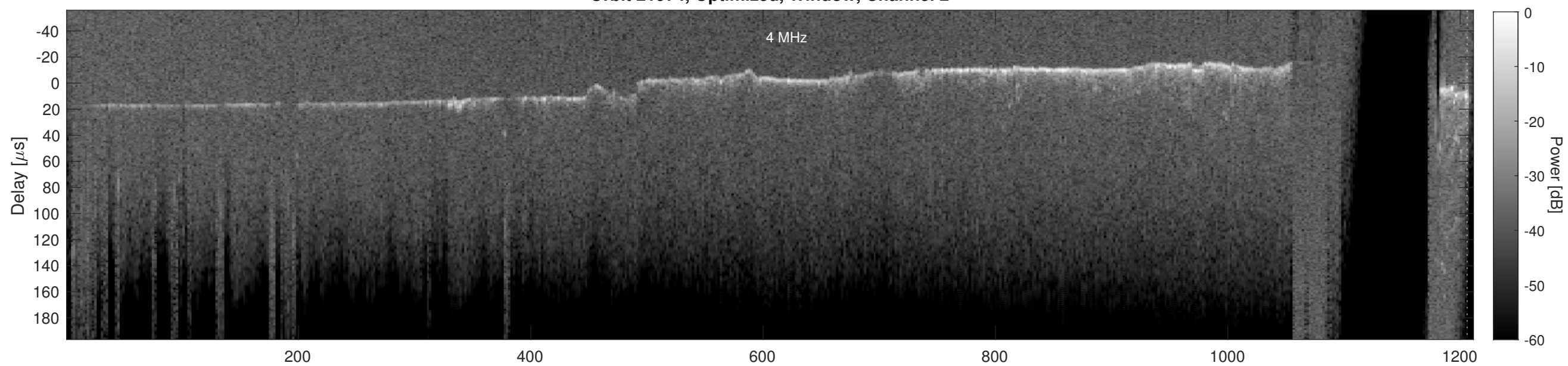
Orbit 21974, Cluttergram
