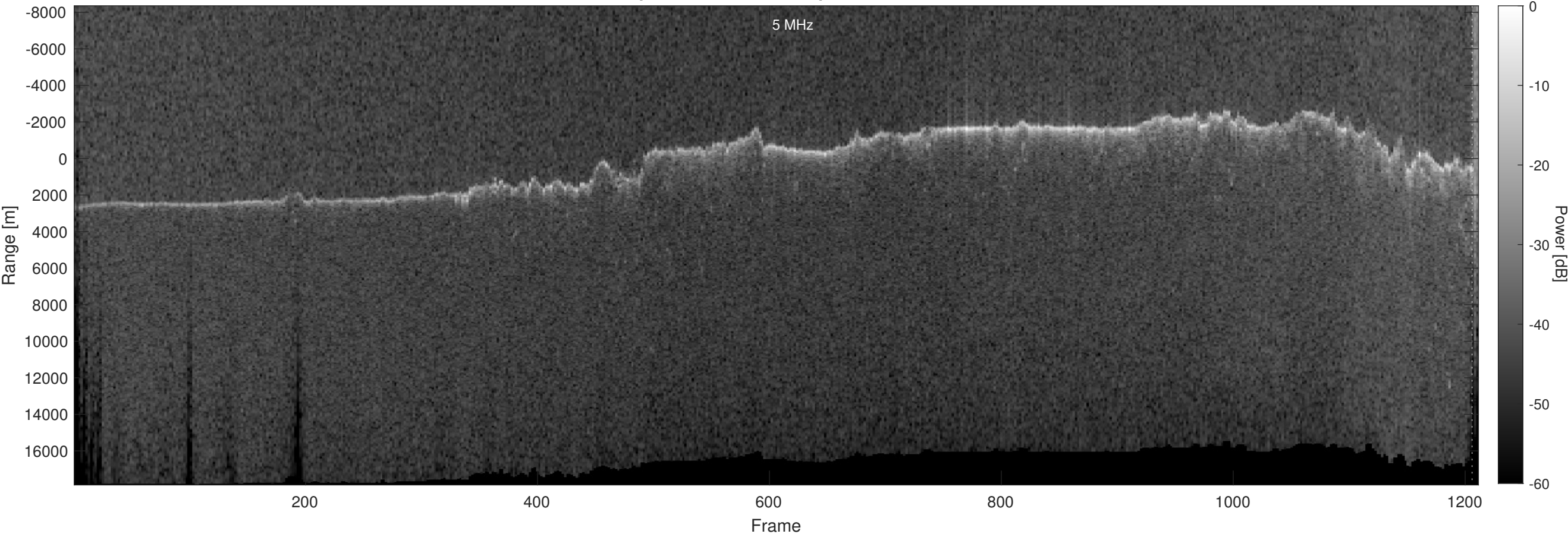
Orbit 21974, Optimized, Window, Depth-Corrected, Channel 2
