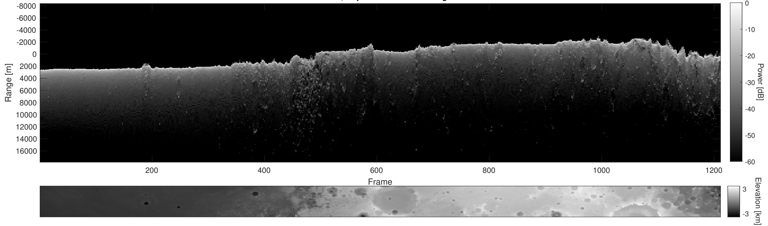
Orbit 21974, Depth-Corrected Cluttergram
