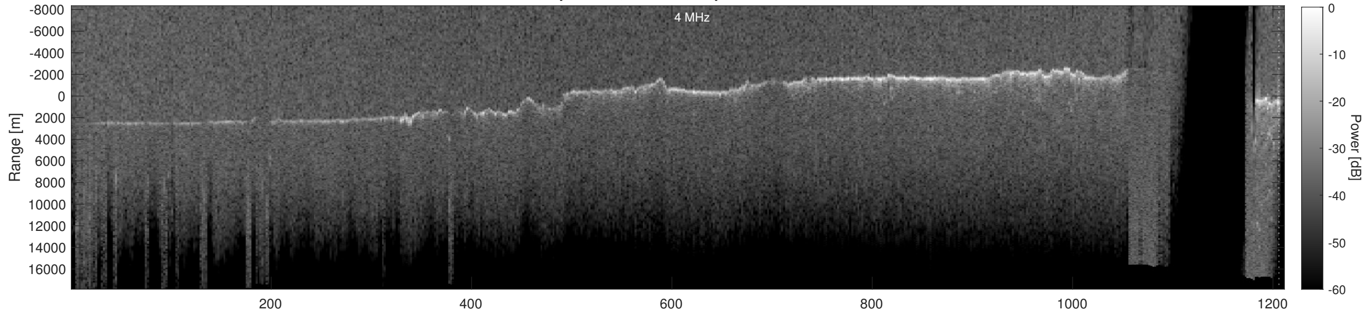
Orbit 21974, Depth-Corrected Cluttergram
