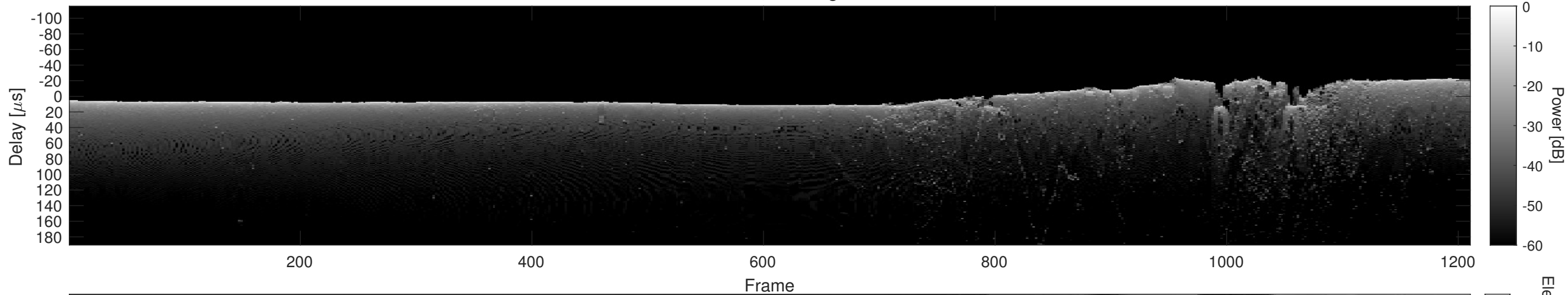
Orbit 21975, Cluttergram
