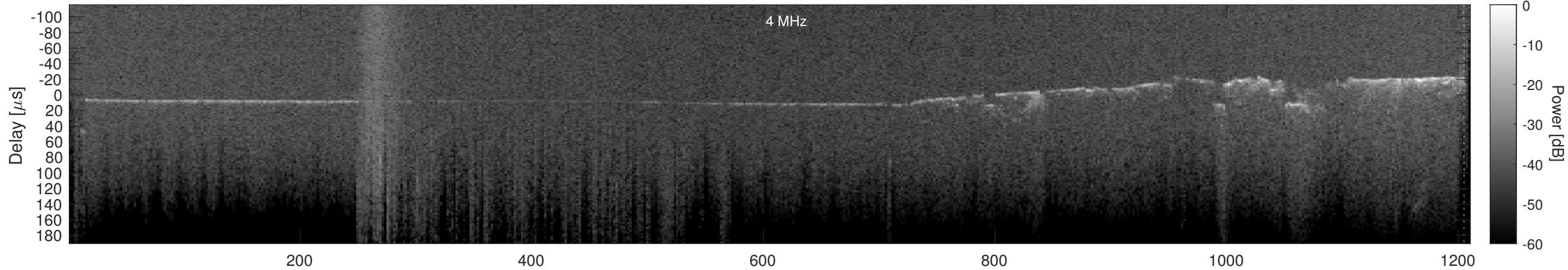
Orbit 21975, Cluttergram
