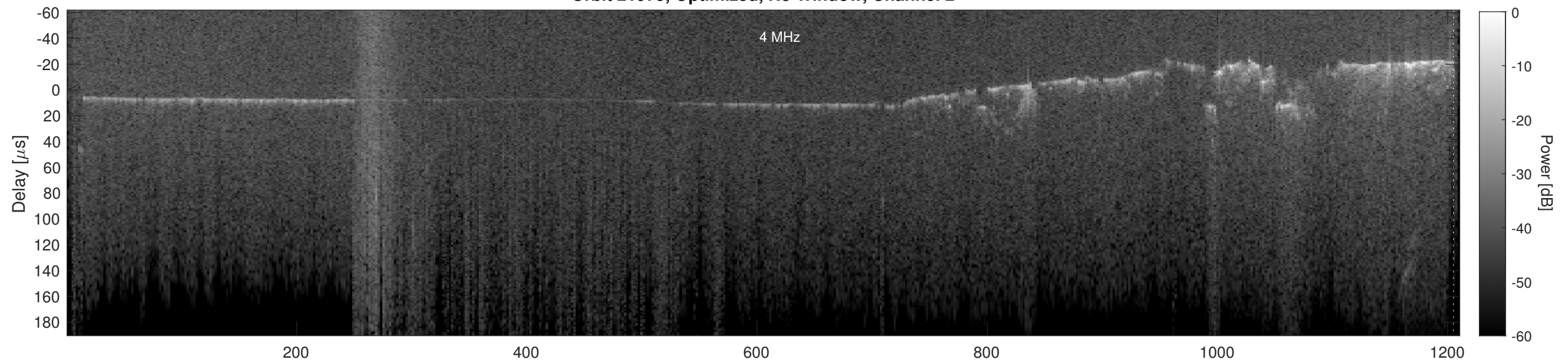
Orbit 21975, Cluttergram
