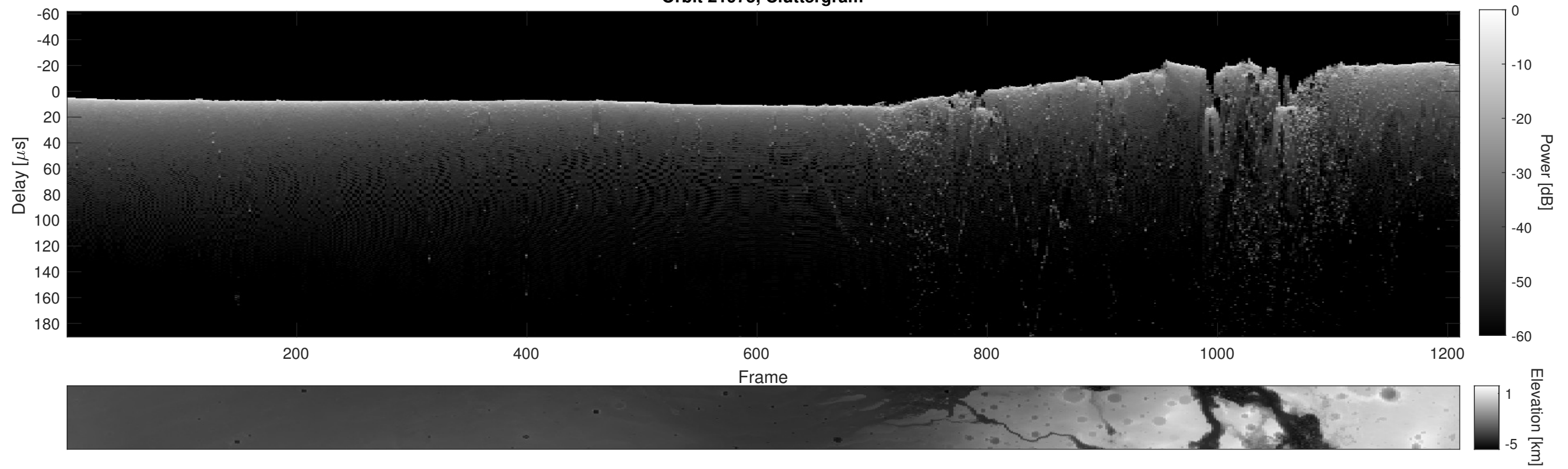
Orbit 21975, Cluttergram
