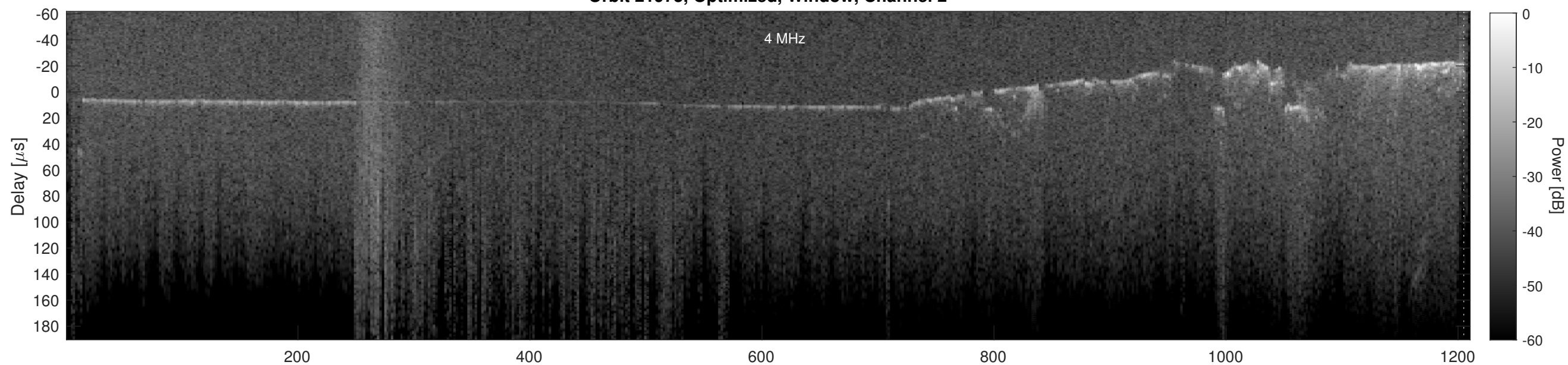
Orbit 21975, Cluttergram
