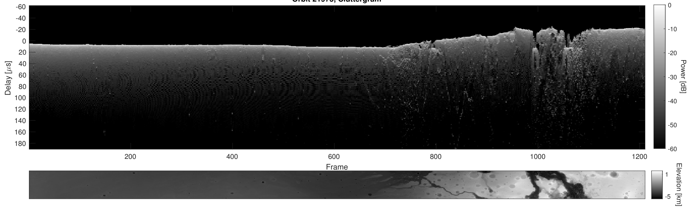
Orbit 21975, Cluttergram
