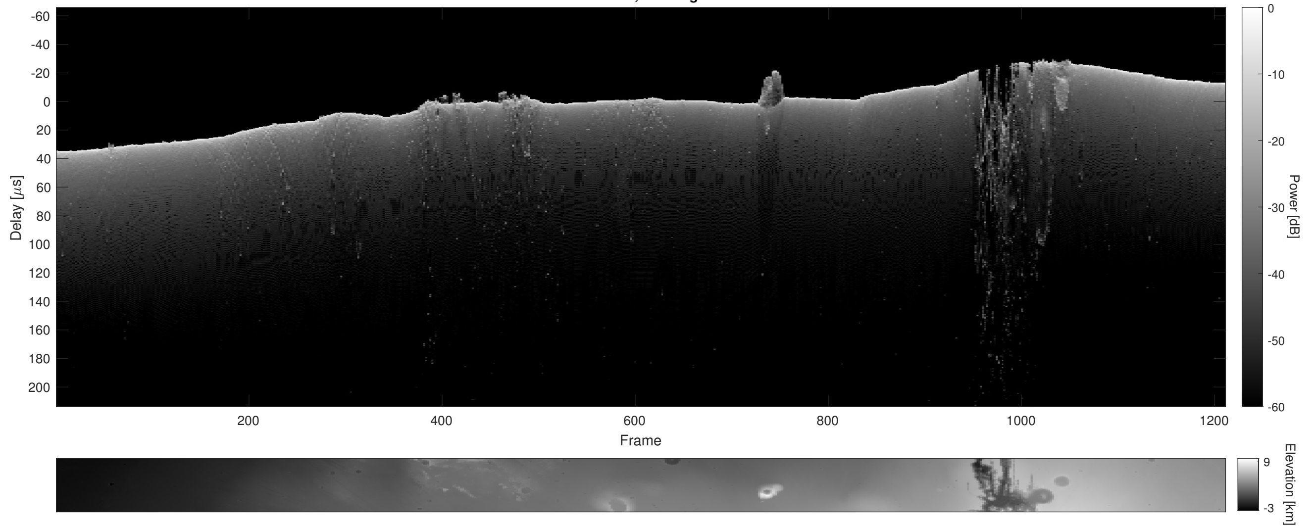
Orbit 21979, Cluttergram
