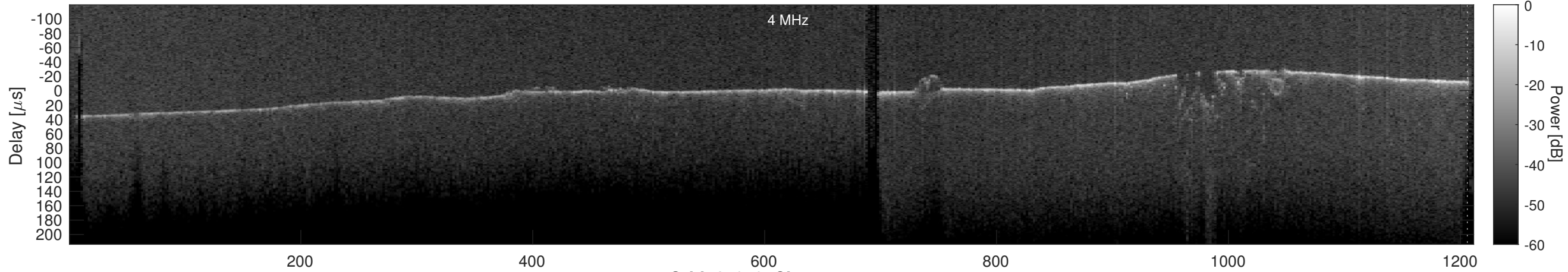
Orbit 21979, Cluttergram
