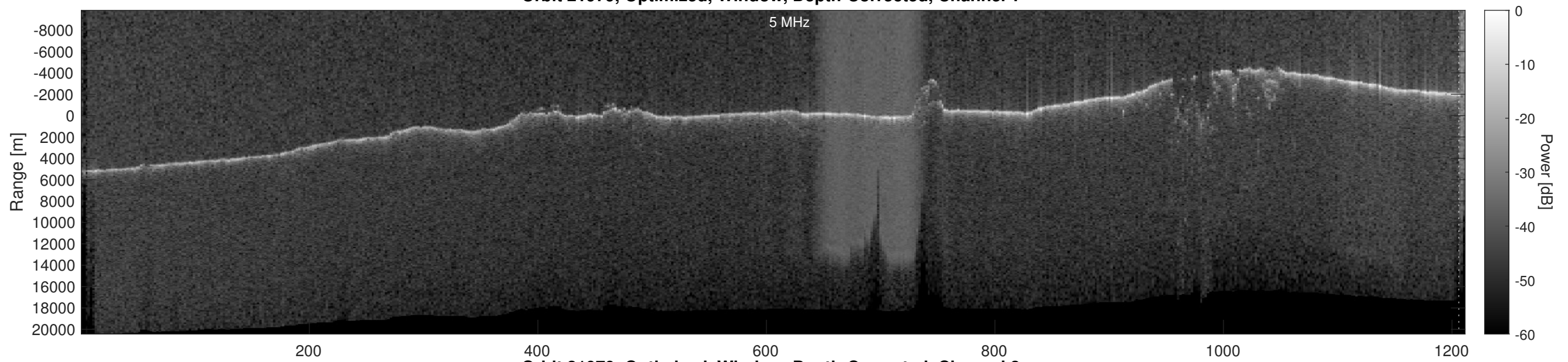
Orbit 21979, Optimized, Window, Depth-Corrected, Channel 2
