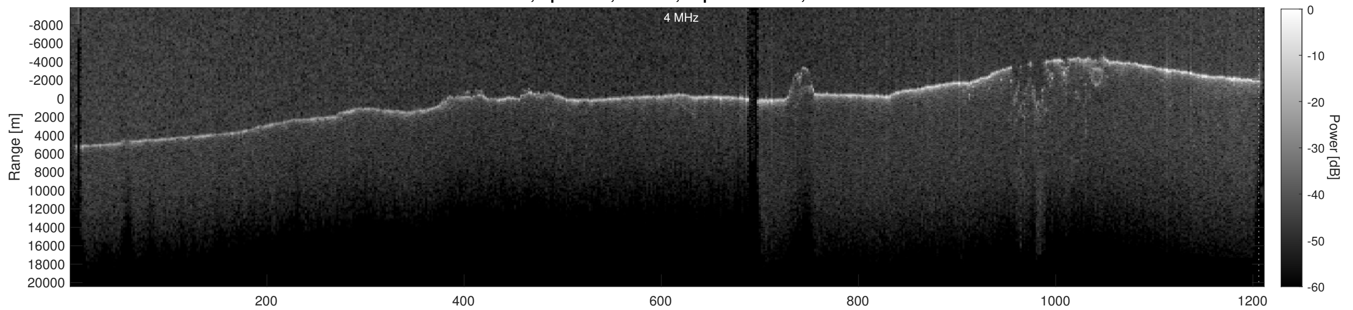
Orbit 21979, Depth-Corrected Cluttergram
