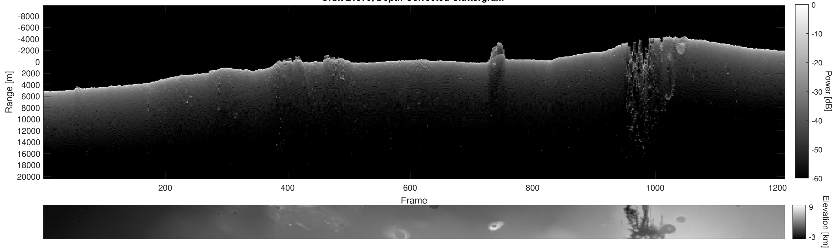
Orbit 21979, Depth-Corrected Cluttergram
