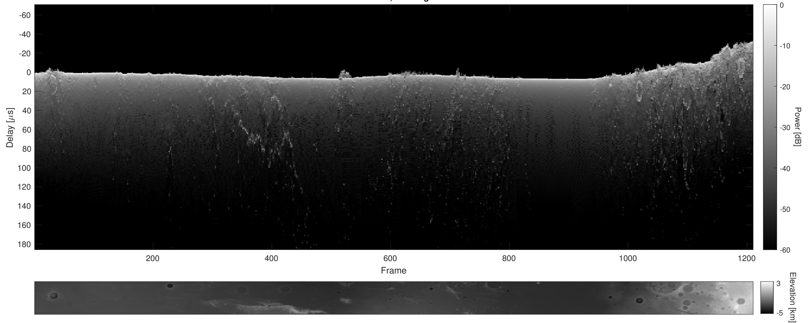
Orbit 21980, Cluttergram
