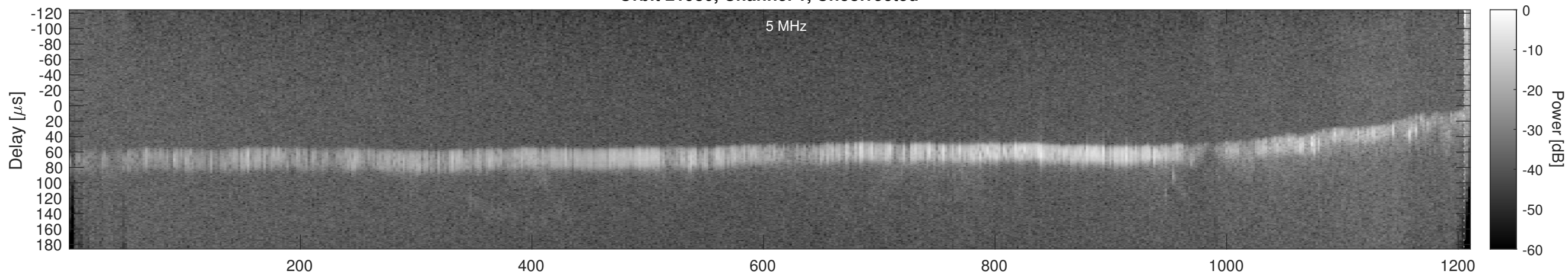
Orbit 21980, Window, Channel 1, Chapman
