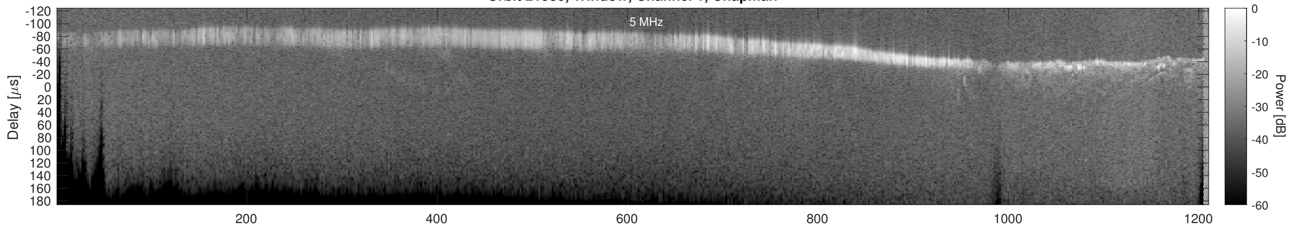
Orbit 21980, Window, Channel 1, Optimized
