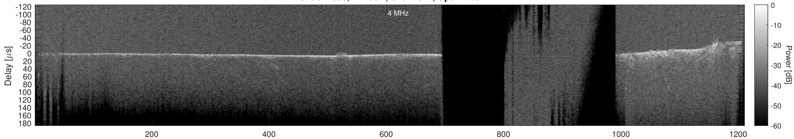
Orbit 21980, Cluttergram
