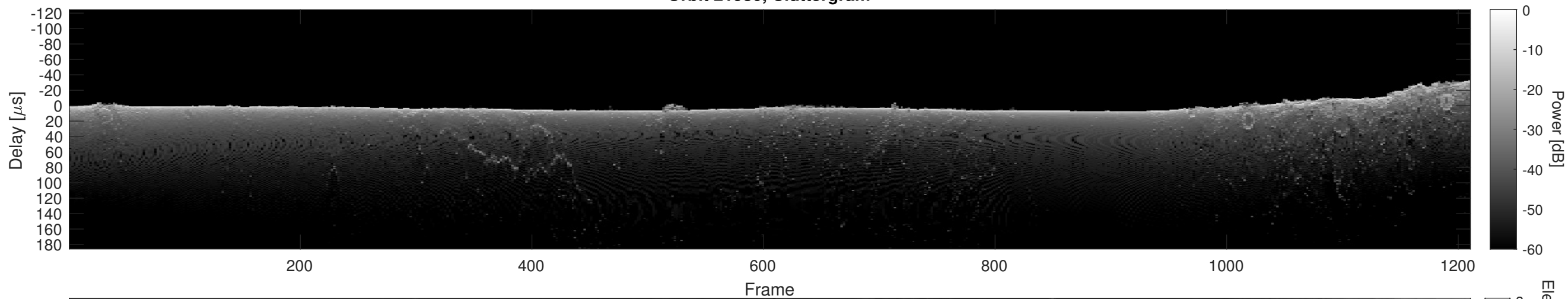
Orbit 21980, Cluttergram
