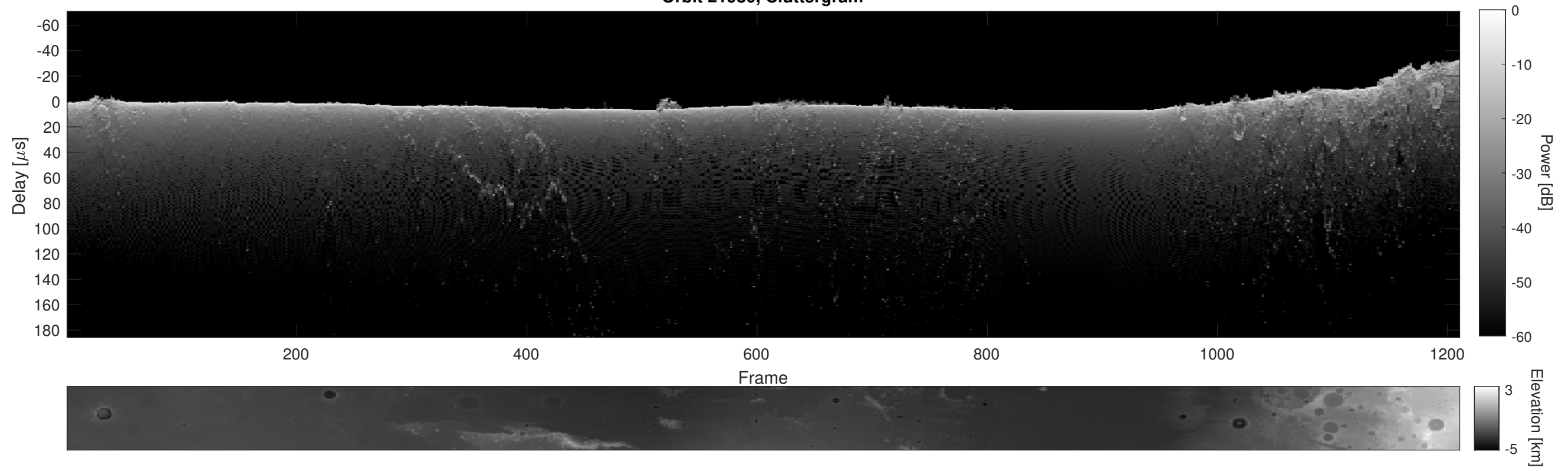
Orbit 21980, Cluttergram
