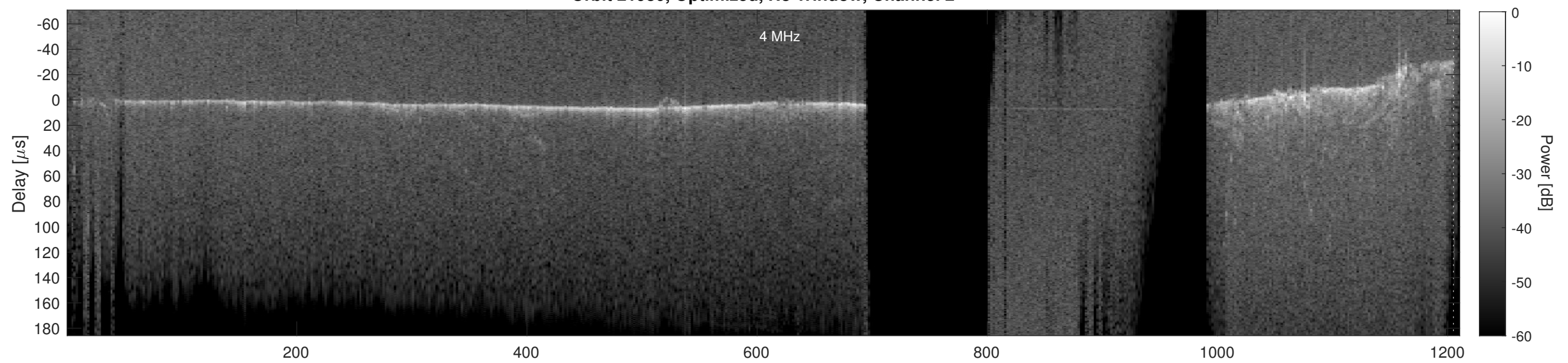
Orbit 21980, Cluttergram
