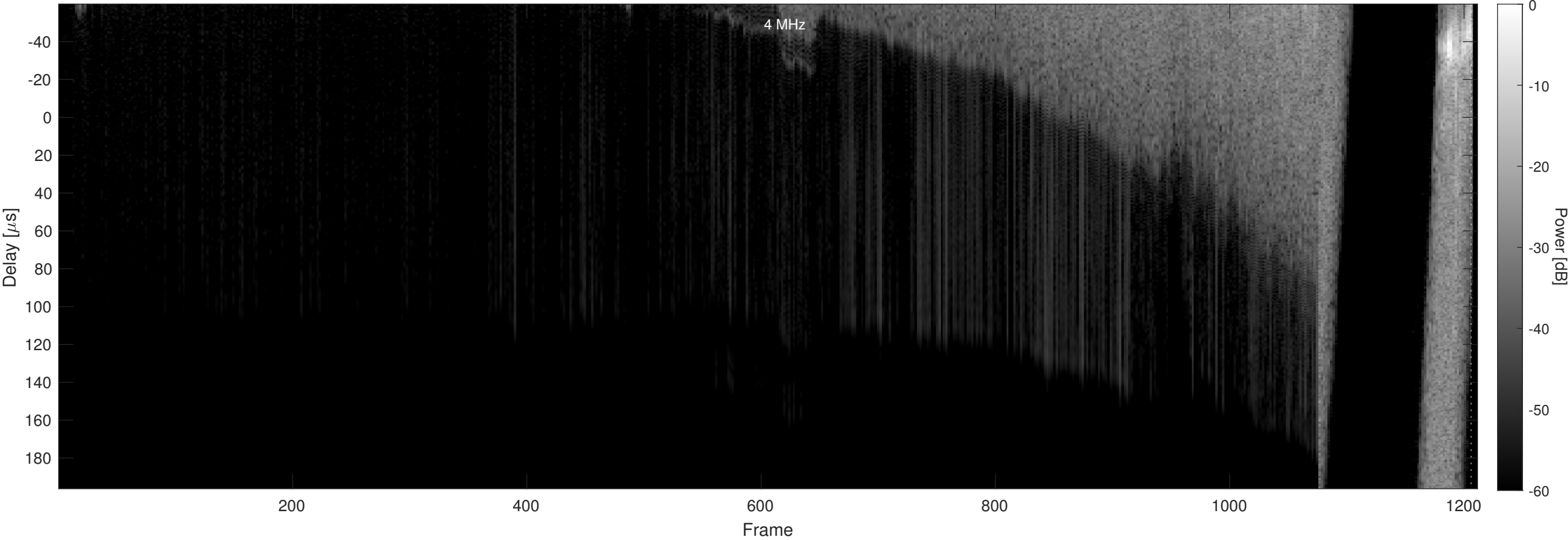
Orbit 21981, Chapman, No Window, Channel 2
