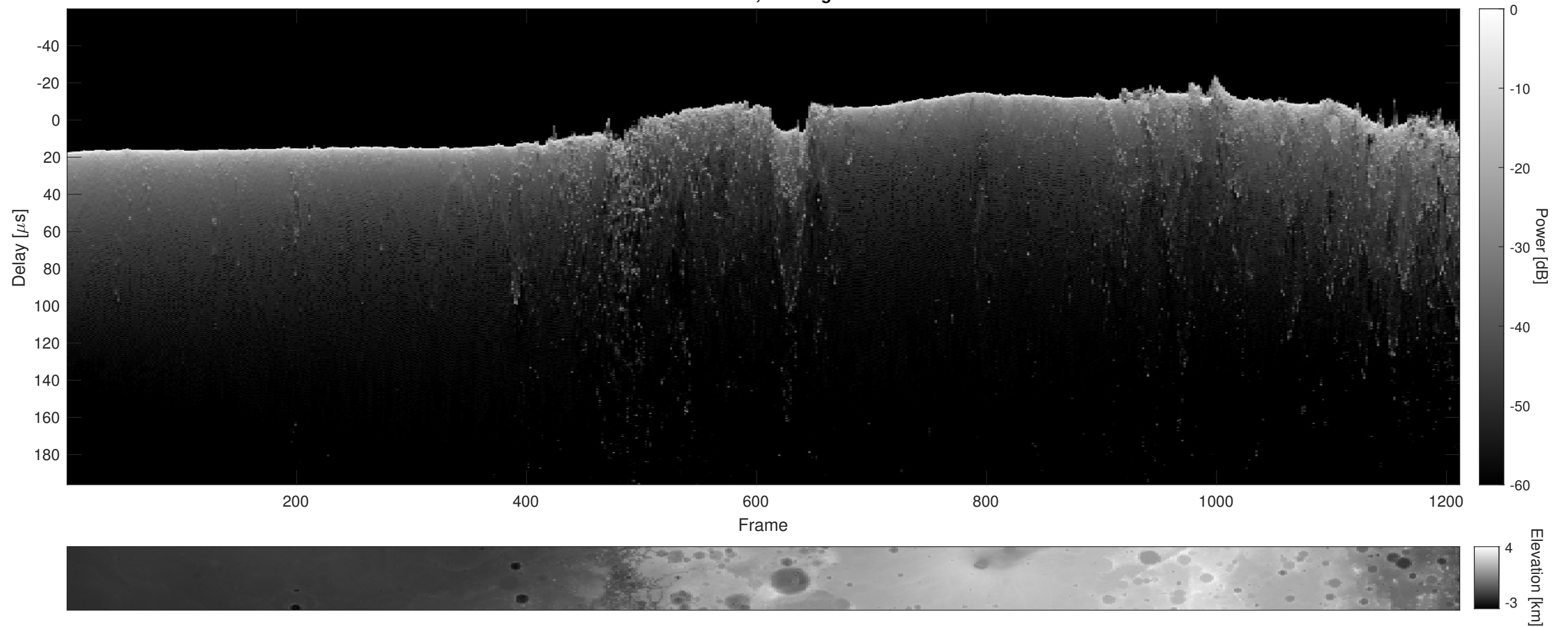
Orbit 21981, Cluttergram
