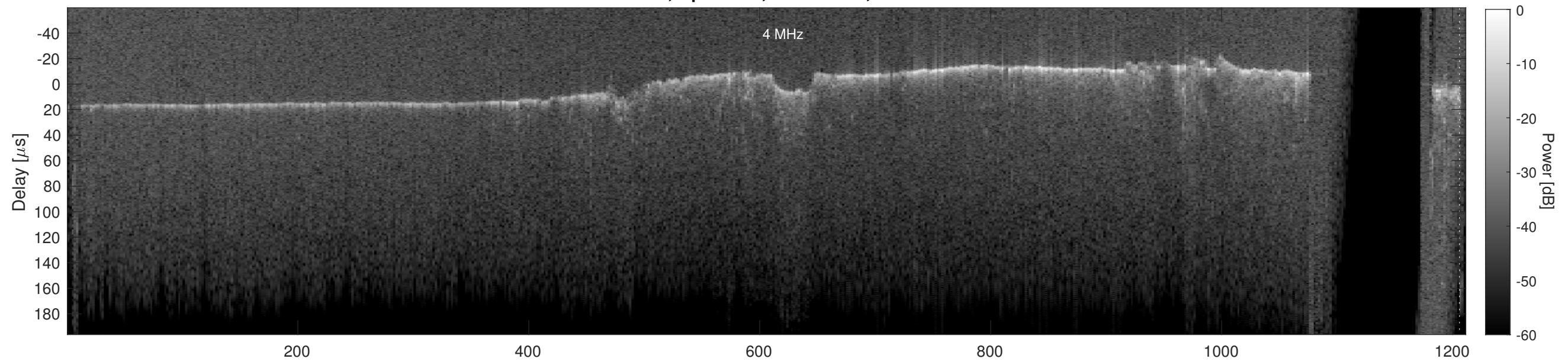
Orbit 21981, Cluttergram
