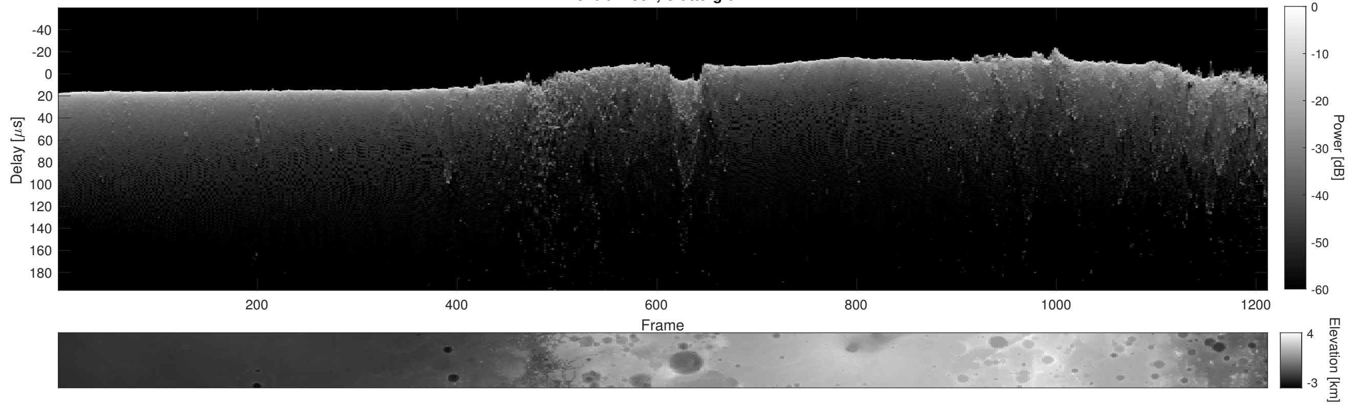
Orbit 21981, Cluttergram
