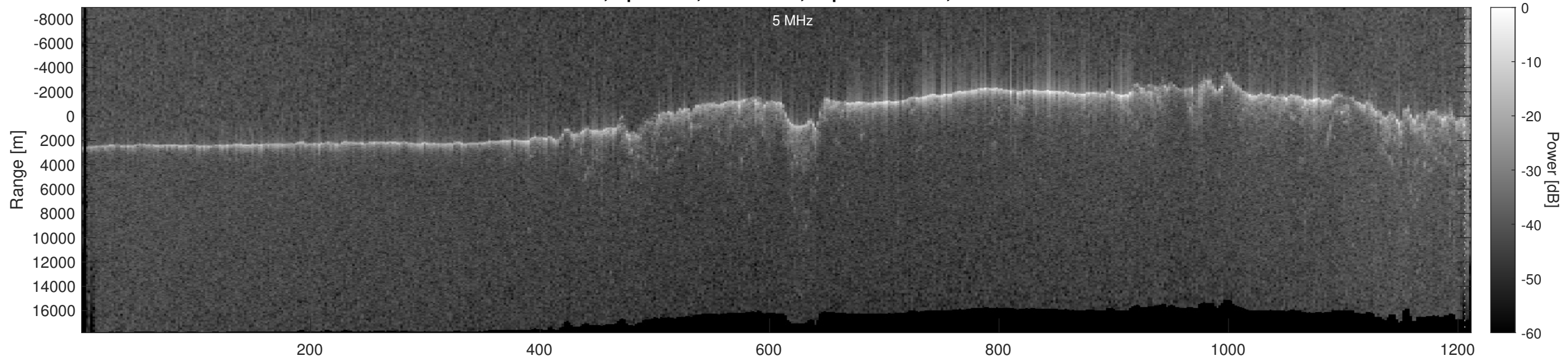
Orbit 21981, Optimized, No Window, Depth-Corrected, Channel 2
