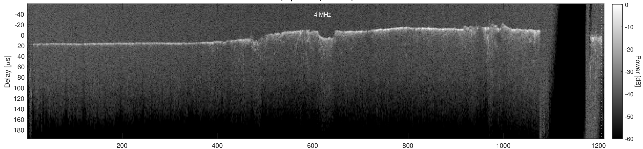
Orbit 21981, Cluttergram
