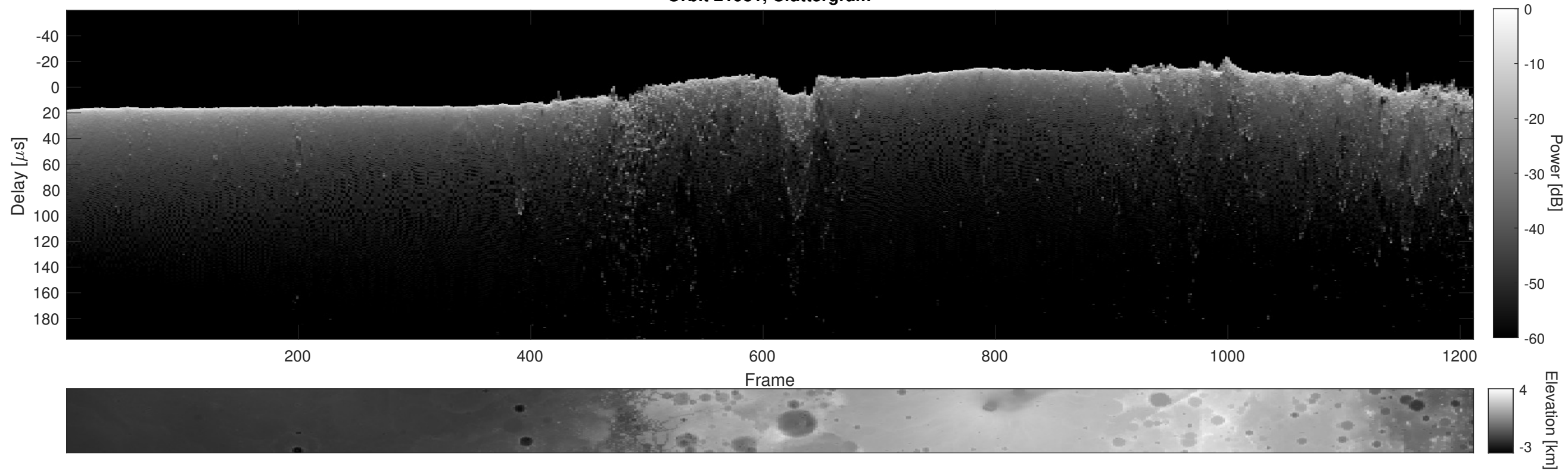
Orbit 21981, Cluttergram
