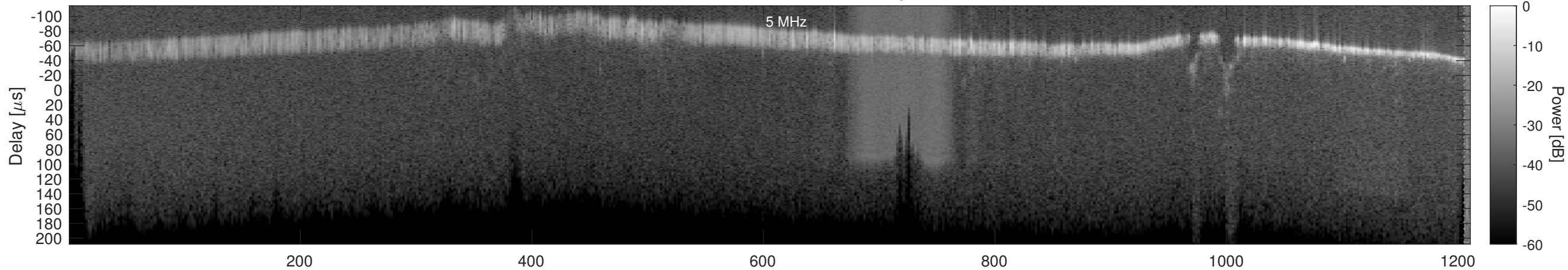
Orbit 21986, Window, Channel 1, Optimized
