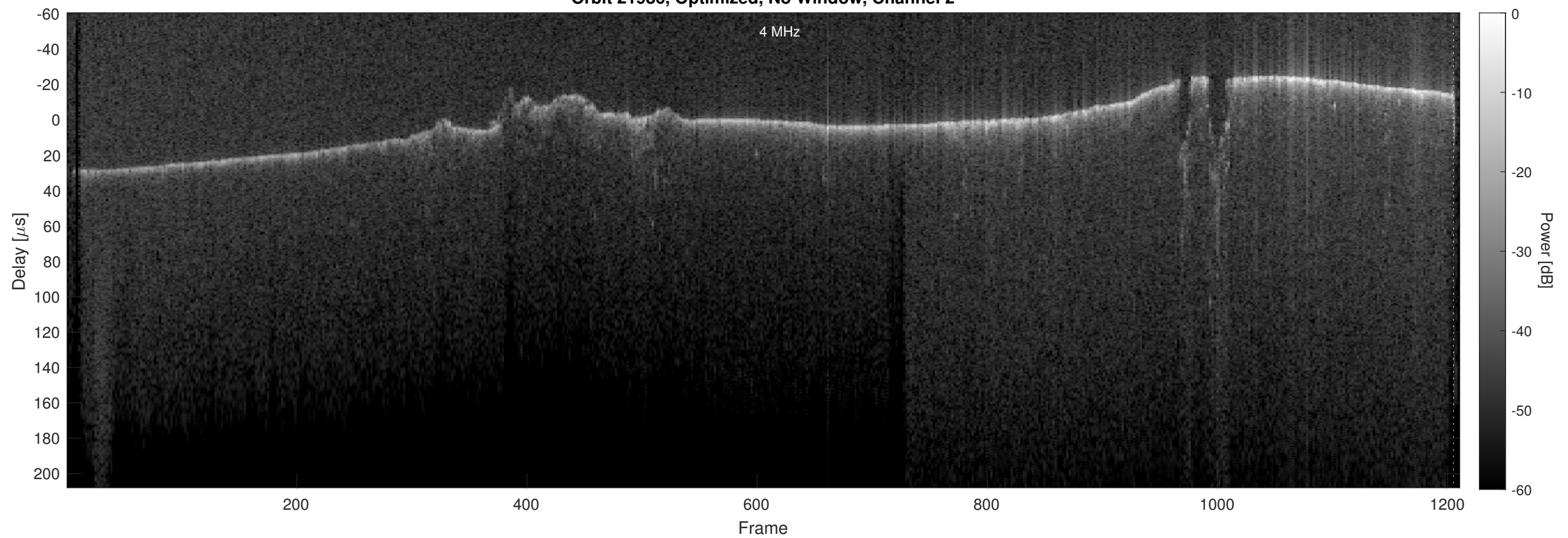
Orbit 21986, Optimized, No Window, Channel 2
