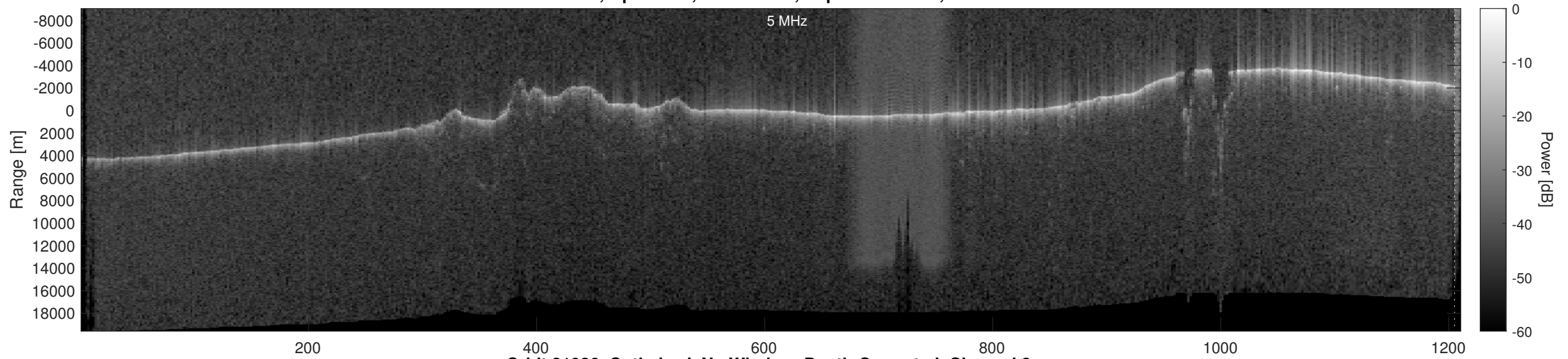
Orbit 21986, Optimized, No Window, Depth-Corrected, Channel 2
