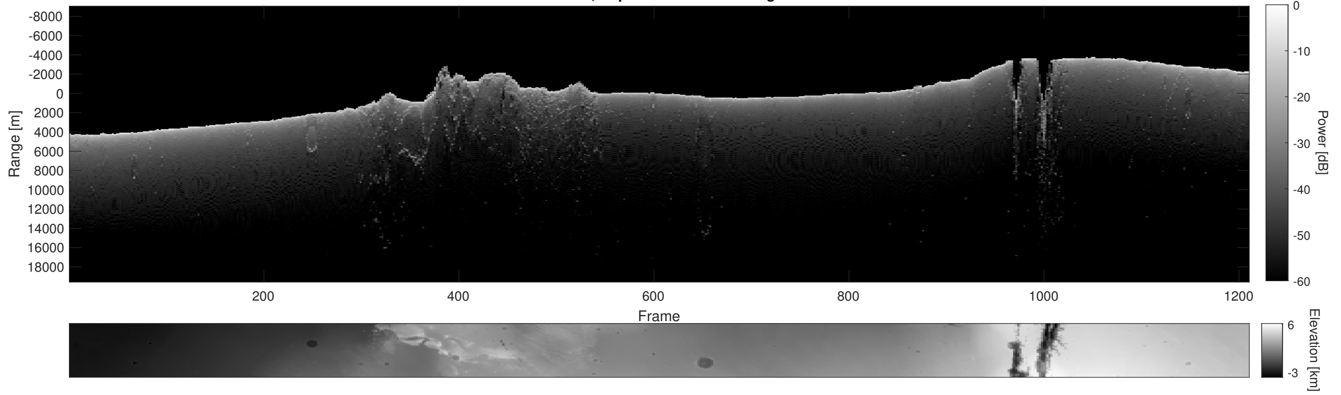
Orbit 21986, Depth-Corrected Cluttergram
