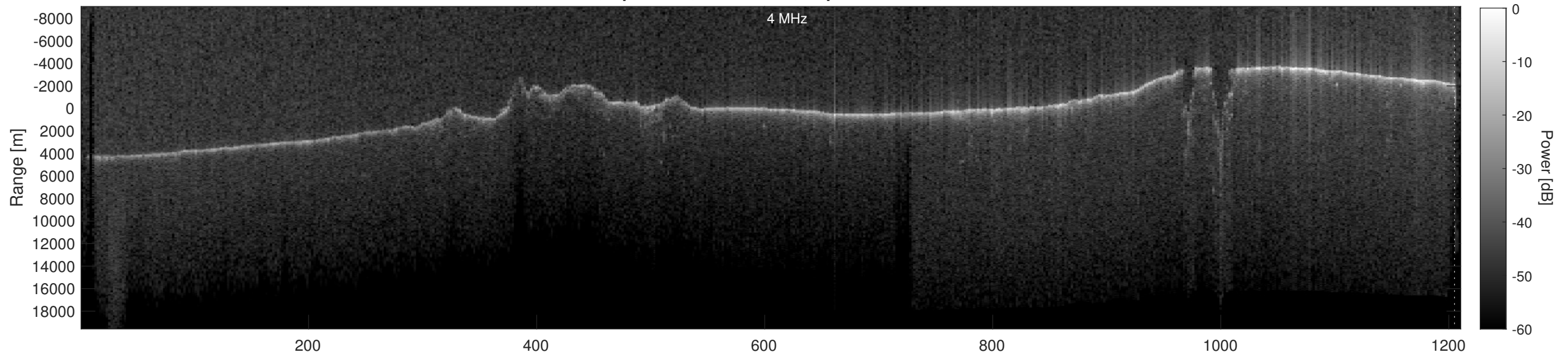
Orbit 21986, Depth-Corrected Cluttergram
