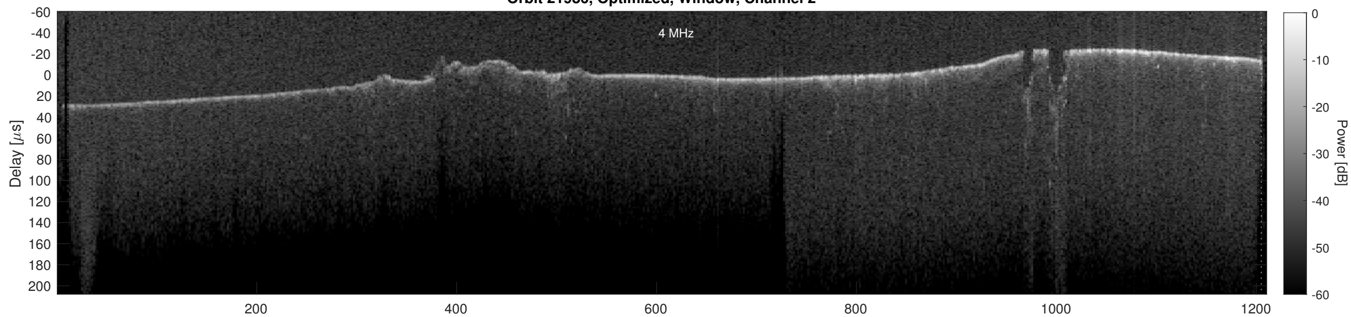
Orbit 21986, Cluttergram
