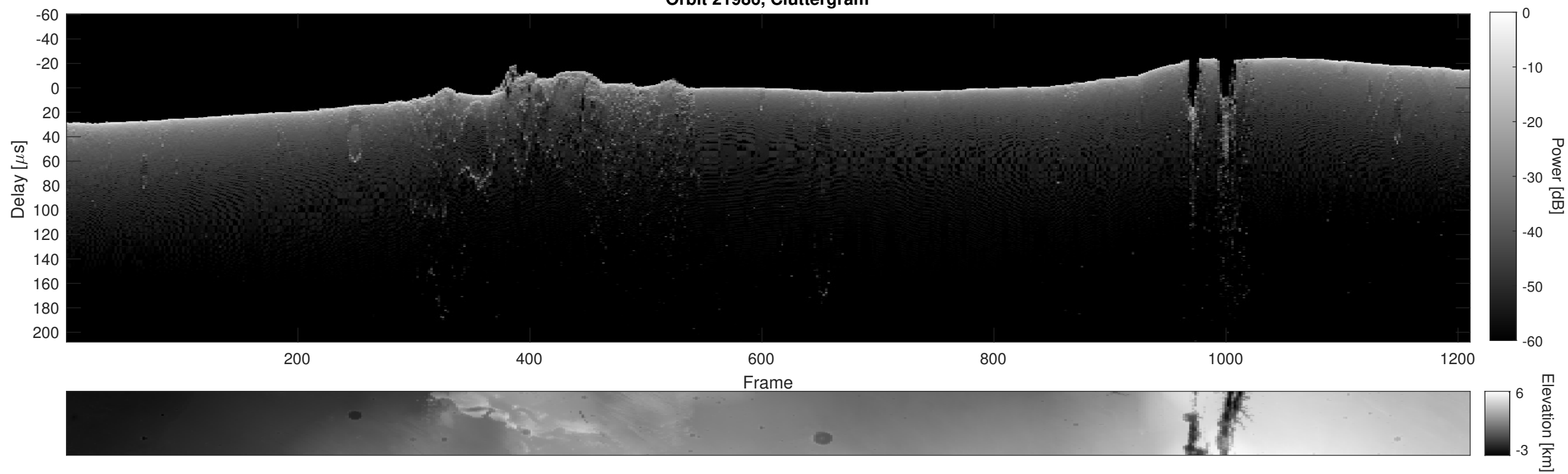
Orbit 21986, Cluttergram
