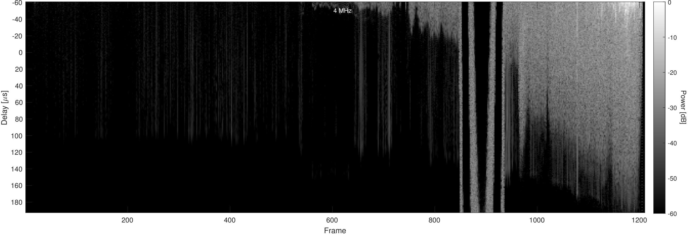
Orbit 21992, Chapman, No Window, Channel 2
